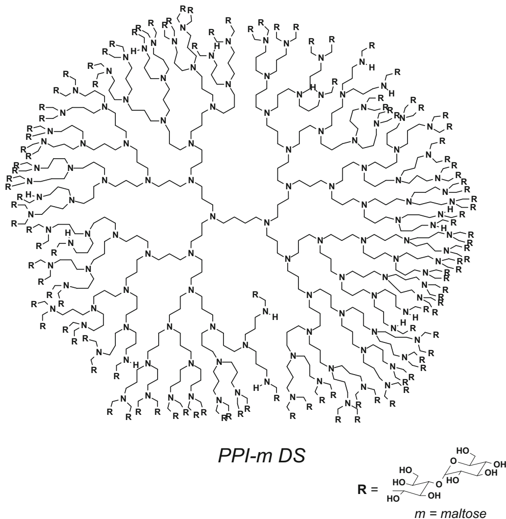
Scheme 1 The structure of PPI dendrimer of the 4th generation modified with maltose
