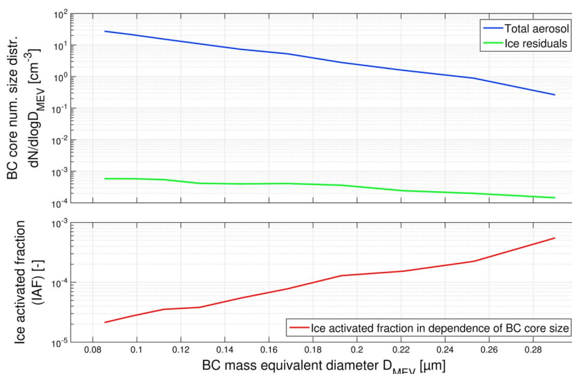
Figure 9. Size distributions of BC cores measured at TI and Ice-CVI and the ice activated fraction for BC-containing particles as a function of rBC mass equivalent diameter, D_{MEV} during CLACE 2013.
