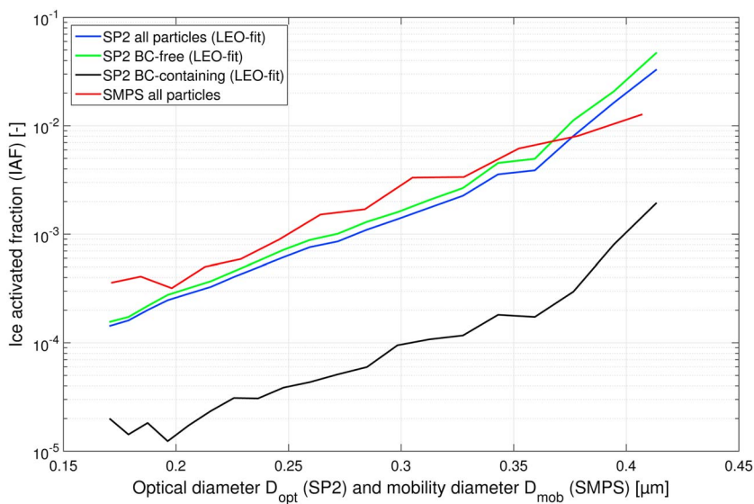
Figure 8. Ice activated fractions (IAF) for BC-free particles, BC-containing particles, and all particles as a function of optical diameter ( D_{opt} ) as inferred from the SP2 data. The IAF of all particles as a function of mobility diameter ( D_{mob} ) as measured by the SMPS during the same periods is shown for comparison. Note that the SP2 measurements shown here only covered a subset of the cloud periods included in Figure 7. This subset turned out to have below-average IAF for all particles, which explains the difference between the SMPS results shown here as compared to those shown in Figure 7.
