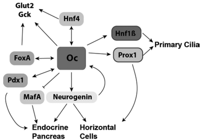
Figure 2. Network of Oc factor targets and associated processes
