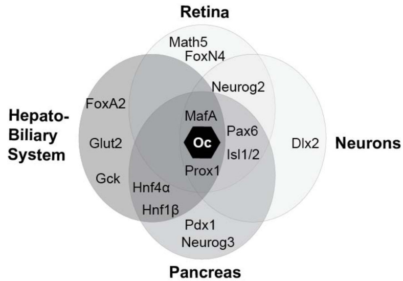
Figure 3. Common targets and co-factors of Oc factors
