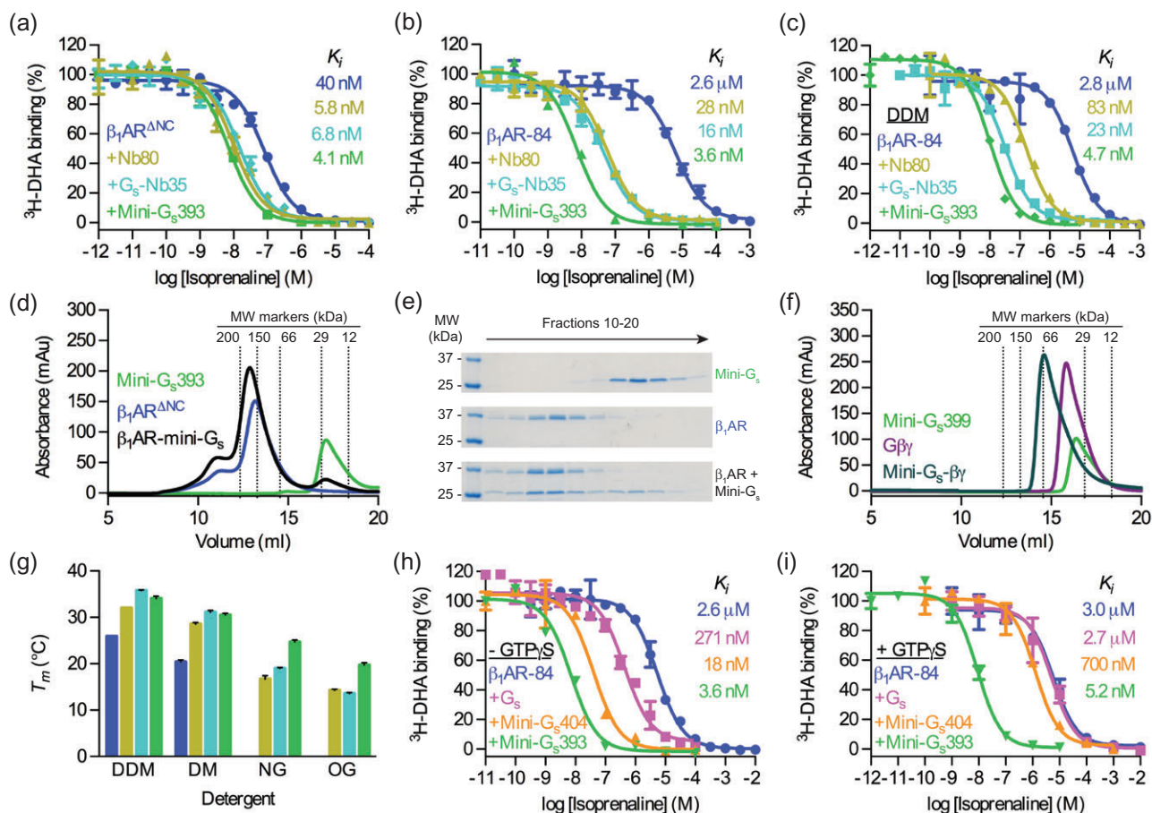
Fig. 3 Validation of mini-G s (a–c) A competition binding assay was used to measure the change in affinity ( K_i ) of isoprenaline induced by Nb80, G s -Nb35, or mini-G s 393 coupling to: (a) membrane-embedded \beta_1\text{AR}^{\text{ANC}} , (b) membrane-embedded \beta_1\text{AR-84} and (c) DDM-solubilised \beta_1\text{AR-84} . (d) Analytical gel filtration analysis of \beta_1\text{AR}^{\text{ANC}} binding to mini-G s 393. The apparent molecular weight of mini-G s 393 was 23 kDa (17.1 ml), which compares well with the theoretical value of 27 kDa. The apparent molecular weight of \beta_1\text{AR}^{\text{ANC}} was 139 kDa (13.2 ml), which is consistent with the 45 kDa receptor being associated with a large detergent micelle; the shoulder at 11 ml (> 300 kDa) probably represents aggregated receptor. A mixture of \beta_1\text{AR}^{\text{ANC}} and mini-G s 393 (1.2-fold molar excess) resolved as a predominant peak with an apparent molecular weight of 160 kDa (12.9 ml). The 21 kDa increase in the apparent molecular weight of the \beta_1\text{AR}^{\text{ANC}} -mini-G s 393 complex compared to uncoupled \beta_1\text{AR}^{\text{ANC}} is consistent with mini-G s 393 binding with 1:1 stoichiometry. (e) SDS-PAGE analysis of the gel filtration eluate confirmed the presence of both \beta_1\text{AR}^{\text{ANC}} and mini-G s 393 in the peak fractions. (f) Analytical gel filtration analysis of G \beta\gamma binding to mini-G s 399. The apparent molecular weights of mini-G s 399 (Supplementary Table SIII) and G \beta\gamma were 32 kDa (16.4 ml) and 42 kDa (15.8 ml), respectively, which is in close agreement with the theoretical values of 29 kDa and 46 kDa, respectively. An equimolar mixture of mini-G s 399 and G \beta\gamma resolved as a single peak with an apparent molecular weight of 73 kDa (14.6 ml). The 31 kDa increase in the apparent molecular weight of the mini-G s 399-G \beta\gamma complex compared to G \beta\gamma is consistent with mini-G s 399 binding with 1:1 stoichiometry. (g) Thermostability of detergent-solubilised \beta_1\text{AR}^{\text{ANC}} alone or in complex with Nb80, G s -Nb35, or mini-G s 393, in different detergents (Supplementary Fig. S10). Uncoupled \beta_1\text{AR}^{\text{ANC}} did not survive solubilisation in NG or OG. Colours correspond to those used in (a). (h–i) GTP-mediated dissociation of \beta_1\text{AR-84} complexes, measured by competition binding assay. The response in isoprenaline K_i induced by G s , mini-G s 404 (Supplementary Table SIII), or mini-G s 393 coupling to \beta_1\text{AR-84} was measured in the presence or absence of GTP \gamma S (250 \mu\text{M} ). (a–c, h, i) Data are representative of at least two independent experiments, each performed in duplicate, with error bars \pm SEM. (g) Data represent mean \pm SEM of at least two independent experiments, each performed in duplicate.
