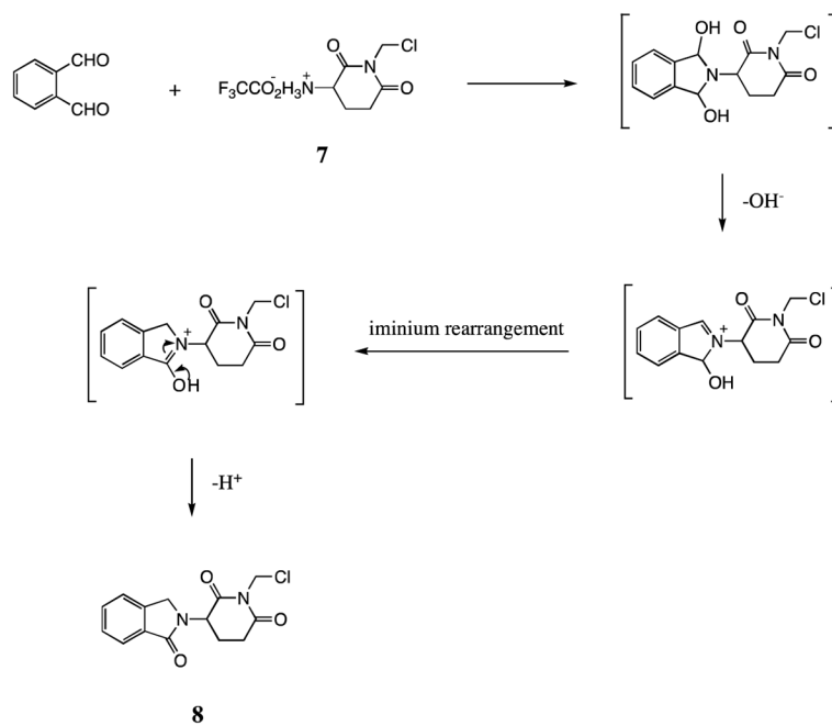
Figure 2. Possible Mechanism Forming Intermediate 8
