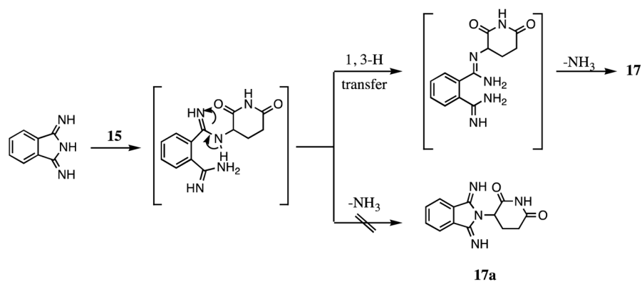
Figure 3. Possible Mechanism Forming Compound 17
