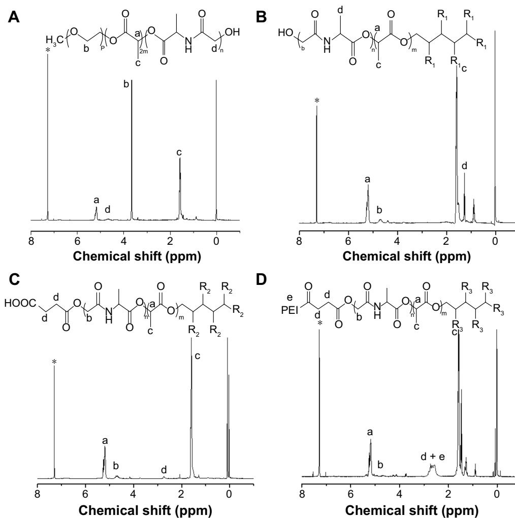
Figure 2 1 H NMR spectra of copolymers.
