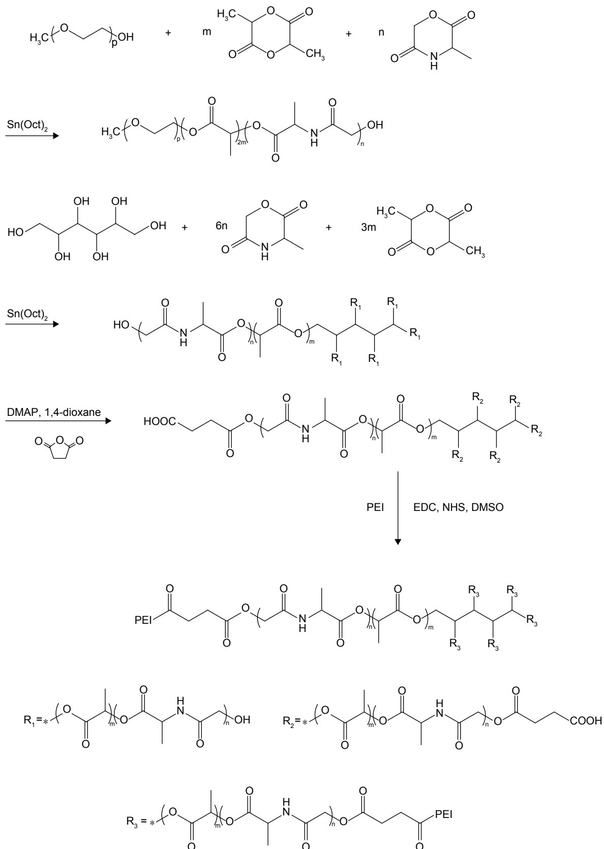
Scheme 2 Synthesis of diblock copolymer mPEG-b-P(MMD-co-LA) and cationic copolymer P(MMD-co-LA)-g-PEI.
