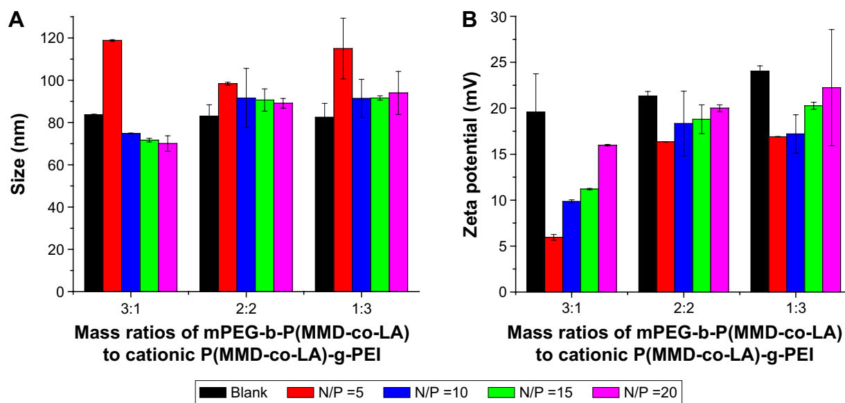
Figure 4 Hydrodynamic diameter ( D_n ) and zeta potential of MPs and MPs/pEGFP-ZNF580 complexes measured by DLS.
