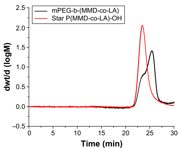
Figure 3 GPC traces of diblock copolymer mPEG-b-P(MMD-co-LA) and star-shaped P(MMD-co-LA)-OH.
