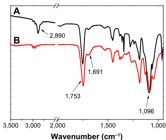
Figure 1 FT-IR spectra (A: copolymer mPEG-b-P(MMD-co-LA); B: star-shaped P(MMD-co-LA)-OH).
