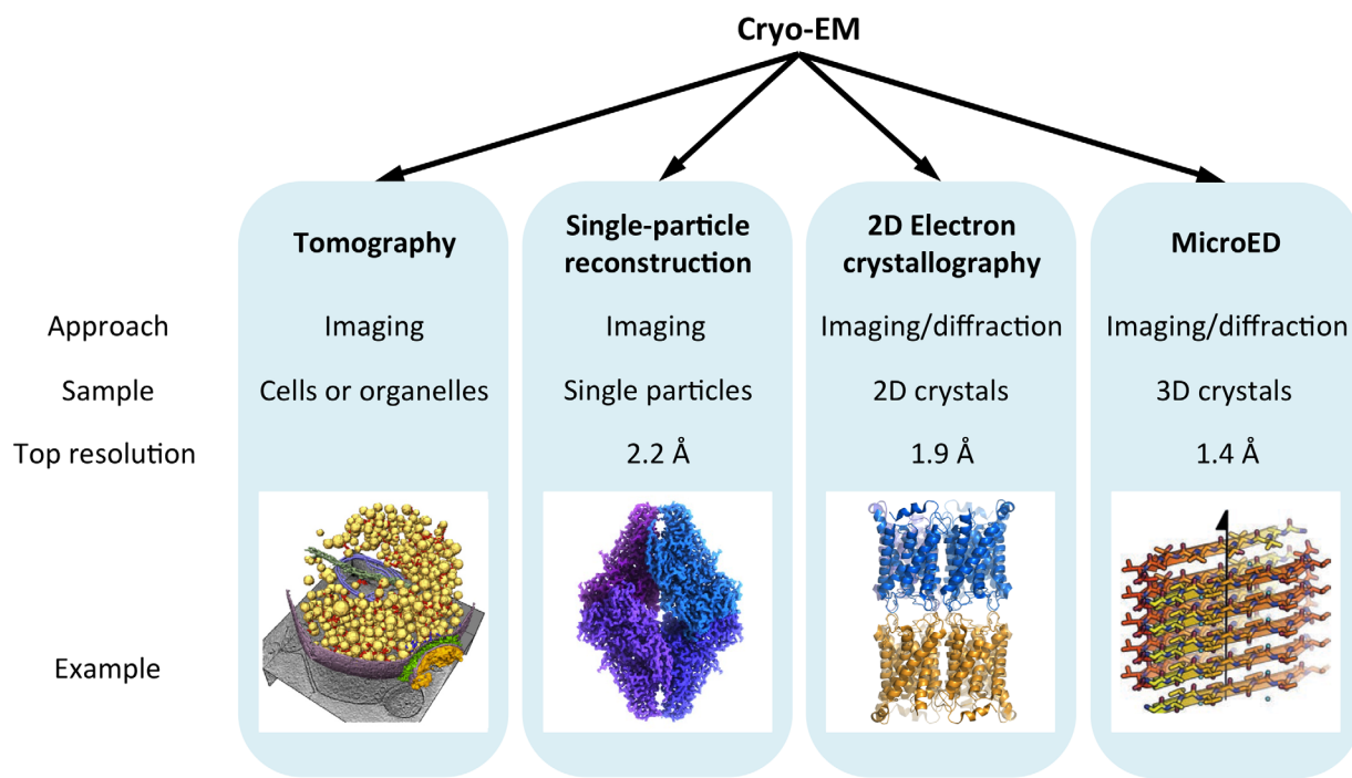
Figure 1. Four methods in Cryo EM. From left to right, a synaptosome model (reprinted from Ref. 3), a 2.2 Å structural model of \beta -galactosidase (reprinted from EMD-2984 entry webpage 4 ), the 1.9 Å resolution model of aquaporin-0, 5 and a 1.4 Å structural model of the \alpha -synuclein NACore stacked in 3D space. 6
