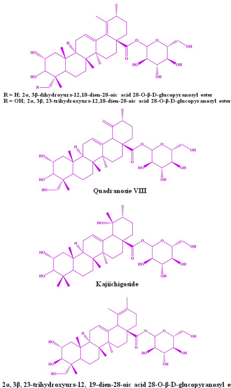
Fig. 2. Structure of ursane triterpenoids isolated from Terminalia arjuna .
