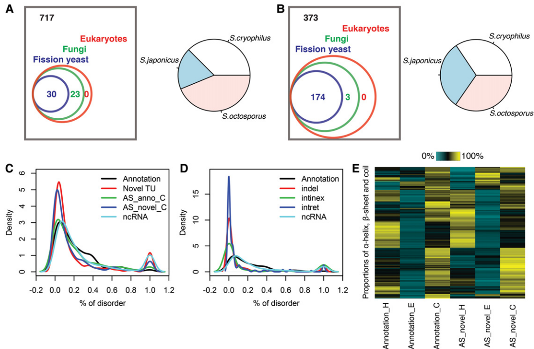
Figure 7. Conservation and secondary structure analysis. (A) Left panel shows the protein BLAST results when using the 770 novel TUs as query sequences. Numbers of novel TUs with alignment hits in different taxa are shown, where the same TU potentially has hits in multiple taxa. Right panel shows the proportion of hits in different fission yeasts. (B) Left panel shows protein BLAST results using as query sequence only the modified part of the 550 protein sequences encoded by AS isoforms. Numbers of AS isoforms with alignment hits in different taxa are shown, where the same AS isoform potentially has hits in multiple taxa. Right panel shows the proportion of hits in different fission yeasts. (C) Distribution of percent of disorder predicted by RaptorX (Källberg et al. 2012). Five classes of protein sequences were examined: full length annotated proteins, longest proteins predicted from novel TUs, C terminus amino acid sequence starting at the first alteration in AS isoforms and its annotated counterpart, and longest proteins predicted from annotated ncRNA. (D) Distributions of percent of disorder predicted for annotated proteins, amino acids affected by insertions and deletions (indel), intron retentions (intret) and introns in exons (intinex) from AS isoforms, and annotated ncRNA. (E) Proportions of \alpha -helix (H), \beta -sheet (E) and coil (C) predicted from C terminus amino acid sequence starting at the first alteration in AS isoforms and its annotated counterpart.
