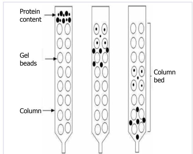
FIGURE 3. Gel-permeation (molecular sieve) chromatography.
