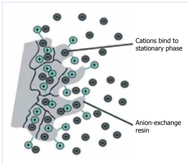
FIGURE 2. Ion- exchange chromatography.
