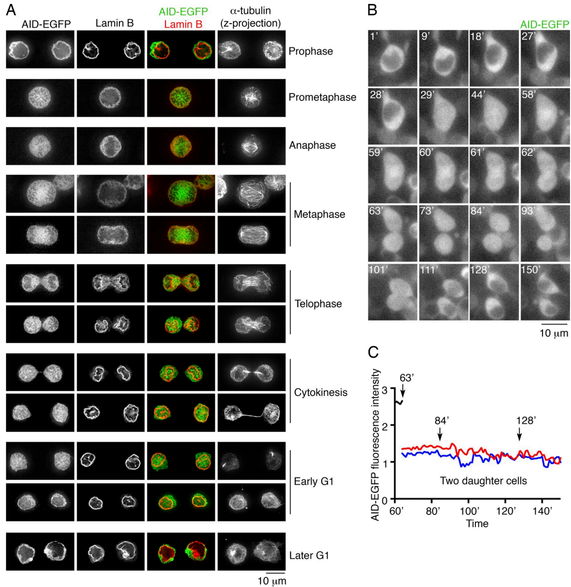
Figure 1. AID accesses the genome during mitosis, cytokinesis, and a short time period in the early phase of G1. (A) Subcellular localization of AID-EGFP from mitosis to G1. AID-EGFP (green) and Lamin B (red, nuclear envelope) are represented by single optical slices (35–40 z-slices each cell). A projection of all slices of \alpha -tubulin shows the microtubule network. The combination of nuclear envelope and microtubule network allows determination of the cell cycle stage. Bar, 10 \mu m. Three independent experiments. (B) Time-lapse imaging of AID-EGFP-expressing B cells during cell division (see Video 1). Single optical z-slices are shown for each time point (indicated in minutes in the top left corner). Bar, 10 \mu m. Two independent experiments were performed. (C) Relative fluorescence intensity of AID-EGFP after cell division. Total AID-EGFP fluorescence was measured over time, and no significant changes in total fluorescence are recorded in the daughter cells (red and blue lines).
