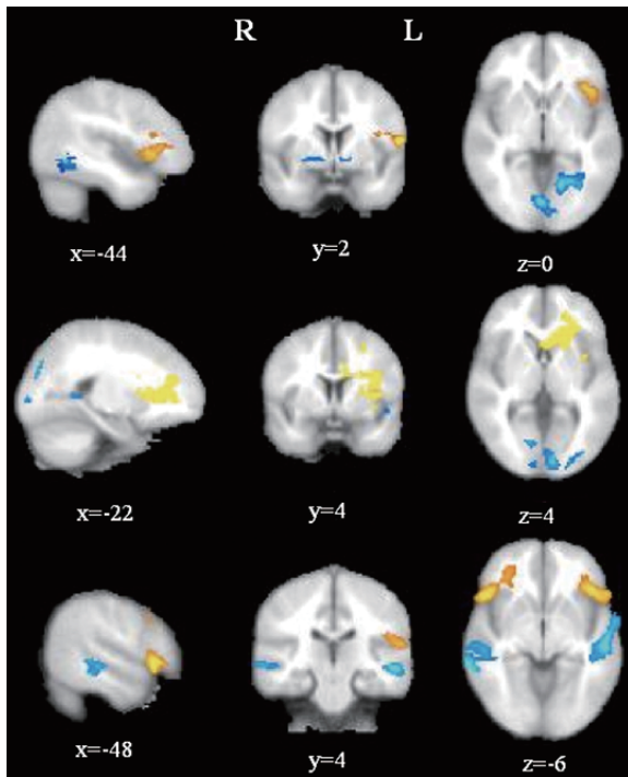
Fig. 3. Age-related activations visual (top), verbal (middle) and auditory (bottom) working memory tasks. Hot colors (red-yellow) point to positive activations and cold colors (blue-cyan) negative activations for each contrast. Sagittal sections show left hemisphere. All maps are thresholded at a whole-brain corrected P < 0.05 using cluster-wise P < 0.05 . For details see Table 3.
