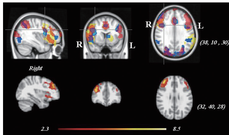
Fig. 2. Top: Group activation map for the visual (red), verbal (blue) and auditory (yellow) working memory in all subjects (both groups). Bottom: Combined task analysis that shows frontal regions as shared activation across the tasks. Numbers in parentheses indicate “x,” “y” and “z” levels on sagittal, coronal, and axial sections.
