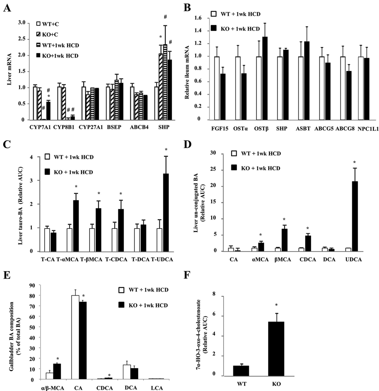
FIGURE 5. HCD-fed Sort1 KO mice had increase bile acid synthesis and altered bile acid composition. Tissues of 1-week HCD-fed mice were used for analysis. A , liver mRNA levels. B , ileum mRNA expression. WT+C , WT plus chow diet; KO+C , knock-out plus chow diet. C and D , hepatic taurine-conjugated and free bile acids (BA) determined by metabolomics analysis. Values in WT mice were set as 1. AUC , area under the curve; T , total. E , bile acid composition in gallbladder bile was analyzed by LC-MS/MS. F , liver 7 \alpha -HO-3-oxo-4-cholestenoate detected by metabolomics analysis. The value in WT was set as 1. All results are expressed as mean \pm S.E. n = 5-6 . * indicates statistical significance, versus WT mice on same diet. # indicates statistical significance, versus chow-fed mice of the same genotype.
