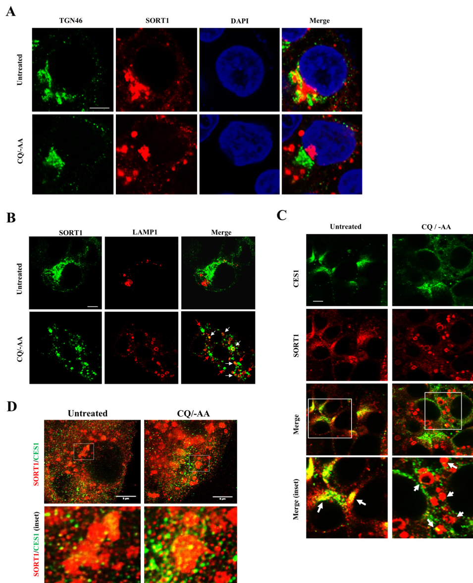
FIGURE 7. SORT1 and CES1 co-localization in HepG2 cells. HepG2 cells were cultured under basal condition or treated with CQ (25 \mu\text{M} ) in amino acid-free Earle's balanced salt solution medium for 3 h. A–C , confocal microscope images. Scale bar: 5 \mu\text{m} . D , STED microscope images. Scale bar: 5 \mu\text{m} .
