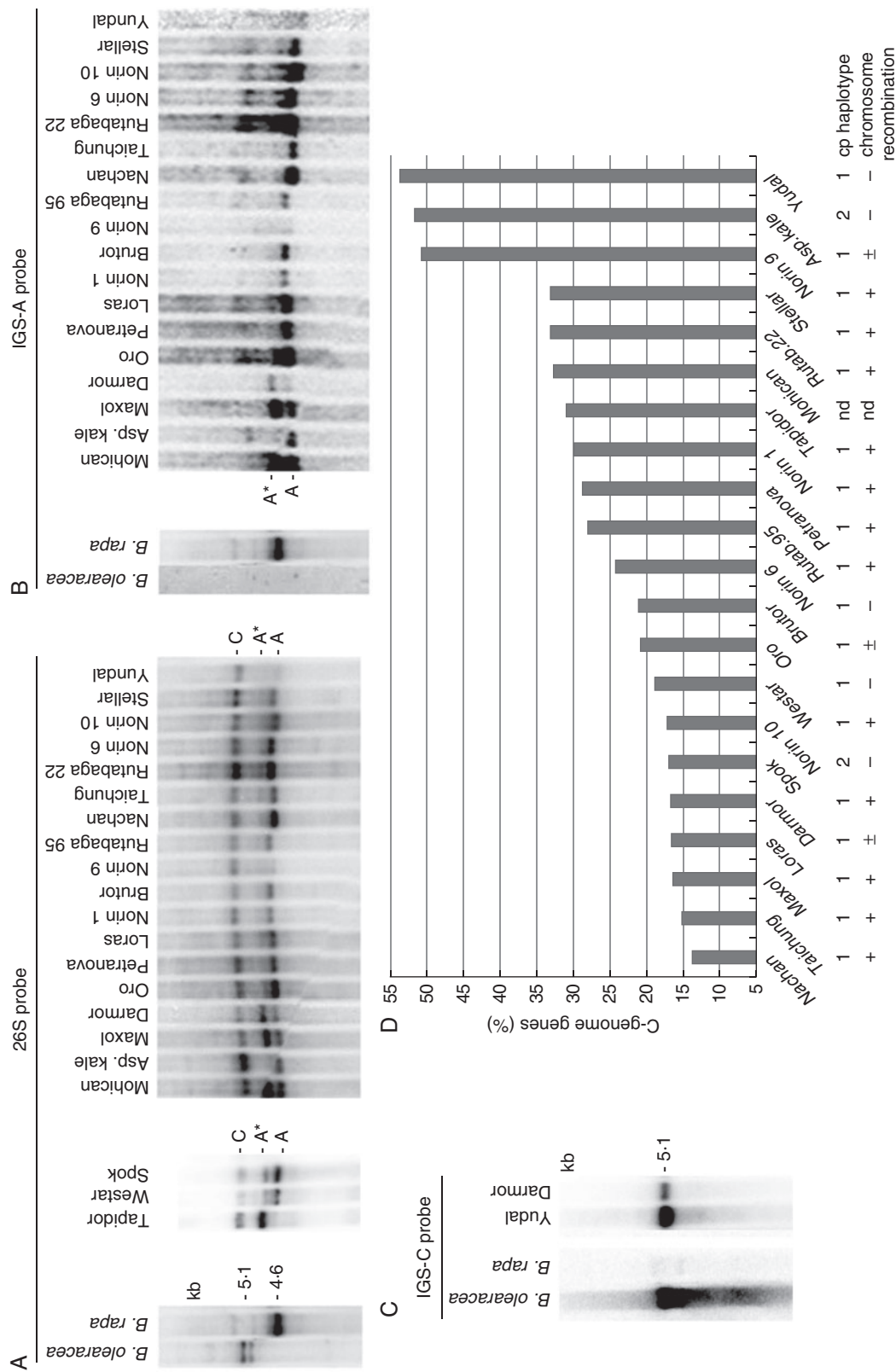
FIG. 1. (A) Southern blot hybridization of genomic DNA from several B. napus cultivars. In the left panel the blot was hybridized with the 26S probe. After stripping the blot was rehybridized with the A-genome-specific IGS probe (B). 'C', C-genome bands; 'A*', A-genome bands; 'A', A-genome bands. (C) Example of a Southern hybridization of the C-genome-specific IGS probe. Note strong hybridization of the probe to 'Yudal' DNA. (D) The radioactivity of bands was quantified using a Phosphorimager and homologue gene number expressed as a proportion of C-genome rDNA to total rDNA. Numbers below indicate two major chloroplast haplotypes identified by Cifuentes et al. (2010). In the same study, the B. napus cultivars were divided into groups with low (-), intermediate (±) and high (+) frequency of homologue chromosome pairing in meiosis (symbols towards the bottom).
