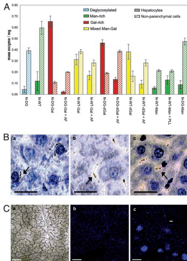
Fig. 3. Cellular localization. (A) Microautoradiographic determination of in vivo cellular localization. The in vivo cell-type localization of ^3\text{H} -labeled enzymes within the liver was determined by microautoradiography in combination with organ distribution data. Sugar-dependent trends emerge. There is a dramatic switch in cell localization from Man-rich N-WT [lane 2, localized predominantly in nonparenchymal cells (hatched bars)] to Gal-rich N-DG-Gal [lane 3, localized predominantly in hepatocytes (filled bars)], which have similar gross organ uptake levels but contrasting cell destinations. (B) Representative microautoradiography images. Liver samples from male Wistar rats dosed with ^3\text{H} -labeled enzymes. Hepatic nuclei are clearly stained dark blue, associated cytoplasm is stained light blue, and sinusoidal regions are pale blue/white. Dark black regions indicate presence of ^3\text{H} -labeled glycosylated enzyme. N-DG-Gal (Ba) localizes predominantly in hepatocyte cytoplasm. In contrast, the predose of AF (N-DG-Gal + AF; Bb) or lack of galactosylation (N-DG; Bc) prevents hepatocyte uptake by the ASGPR and leads to localization in predominantly nonparenchymal cell regions. (Scale bar, 25 \mu\text{m} .) (C) Confocal microscopy. (Ca) Phase image illustrates the architecture of a liver section from an N-DG-Gal-dosed male Wistar rat; plates of hepatocytes surround a central blood vessel. (Cb) Fluorescence image of the same section without MEND-Rha (some collagen-derived autofluorescence is observed). (Cc) Fluorescence image of the same section with prodrug MEND-Rha. Strong fluorescence demonstrates release of MEND in the hepatocyte region. (Inset) Fluorescence image from undosed animal with MEND-Rha. (Scale bar, 0.1 mm.)
