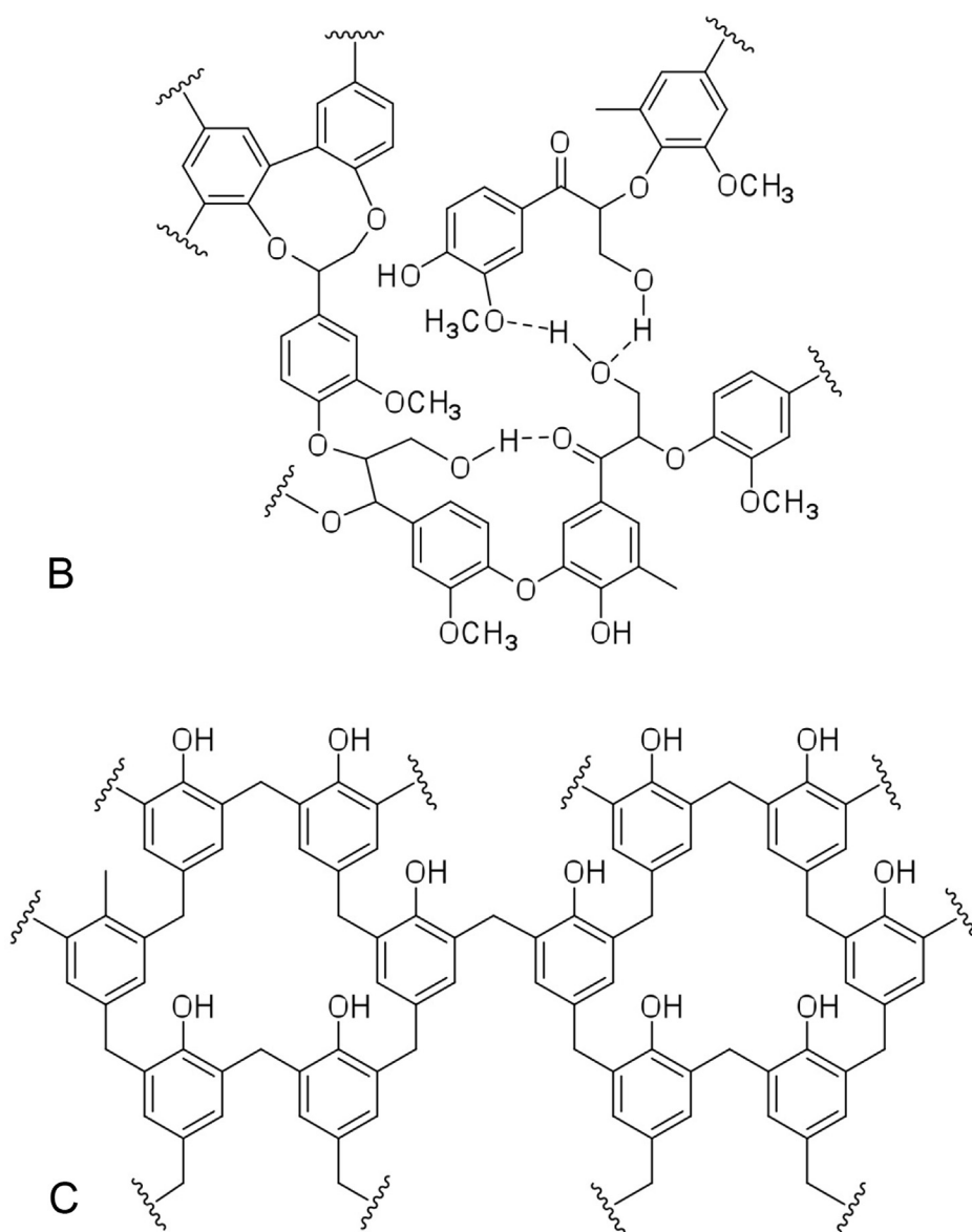
Fig. 6. A. Phanerocheate chrysosporium , a white rot fungus, so-called due to the bleached appearance of wood degraded by such species. B–C. Show the structures typical of lignin and phenol-formaldehyde resins respectively. The structural similarities mean that the natural metabolic capabilities of fungi such as P. chrysosporium can be used to degrade – and therefore recycle – persistent man-made materials such the phenol-formaldehyde resins.
