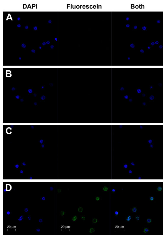
Figure 5 Photograph under confocal microscope of cells incubated overnight with (A) untreated control (RPMI 1640 medium only), (B) RNA control (fluorescent RNA only), (C) Ψ dendriplex at dendrimer:RNA (±) charge ratio =2:1, and (D) Ψ dendriplexes at dendrimer:RNA (±) charge ratio =4:1. Abbreviation: RPMI, Roswell Park Memorial Institute.
