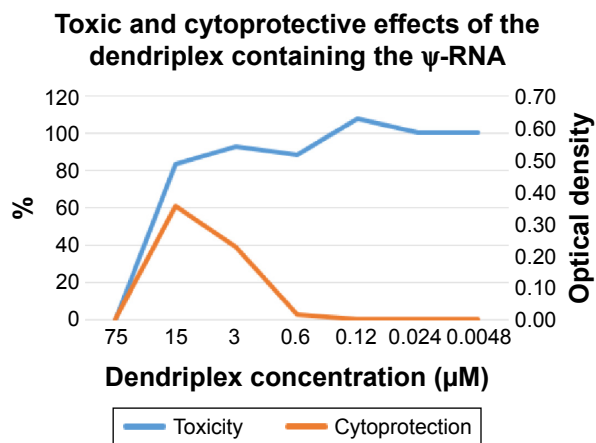
Figure 6 Toxic and cytoprotective effects of the dendriplex (Ψ RNA + dendrimer). Notes: The toxic and cytoprotective effects were determined by exposing uninfected and HIV-infected MT4 lymphocytes, respectively, to serial dilutions of the dendriplex containing the Ψ RNA decoy.
