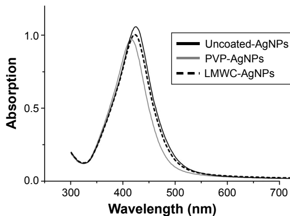
Figure 2 UV-Vis absorption spectra of uncoated-AgNPs (black full line), PVP-AgNPs (gray full line), and LMWC-AgNPs (black dash line). Abbreviations: Uncoated-AgNPs, silver nanoparticles without surface stabilizer; PVP-AgNPs, polyvinylpyrrolidone-coated silver nanoparticles; LMWC-AgNPs, low molecular weight chitosan-coated silver nanoparticles.
