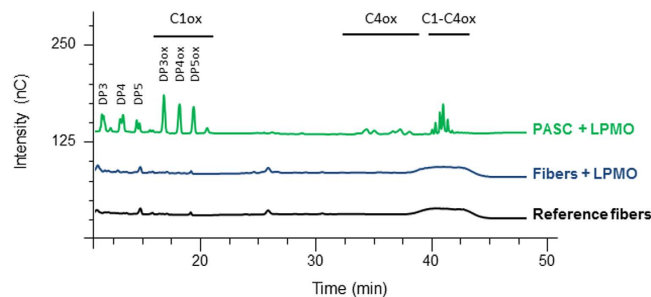
Figure 1. Chromatographic analysis of soluble oxidized cello-oligomers released by the action of LPMO. The chromatograms display the oligomers released from PASC treated with LPMO (green). When cellulose fibers were submitted to LPMO, no release was observed (blue). Reference (black) corresponds to cellulose fibers incubated at the same conditions but in the absence of LPMO. The chromatograms of standard oligomers (DP3–6 and DP oxidized 3–6) are shown in Figure S1.
