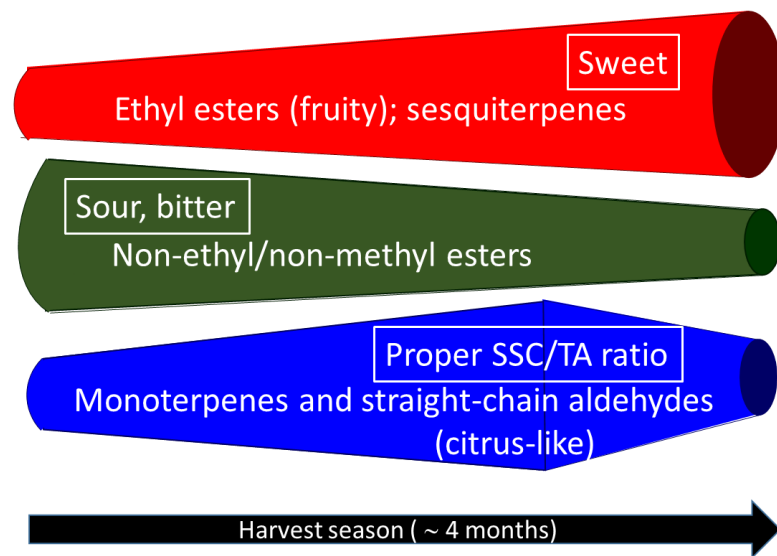
Figure 4. A schematic diagram to demonstrate the change patterns of different non-volatile (boxed) and volatile (non-boxed) flavor chemical compounds along with harvest time (from February/March to May/June) in “Valencia” orange juice. The width of the band indicates the relative abundance of each chemical class/attribute except for SSC/TA ratio which represents the optimal quality.
