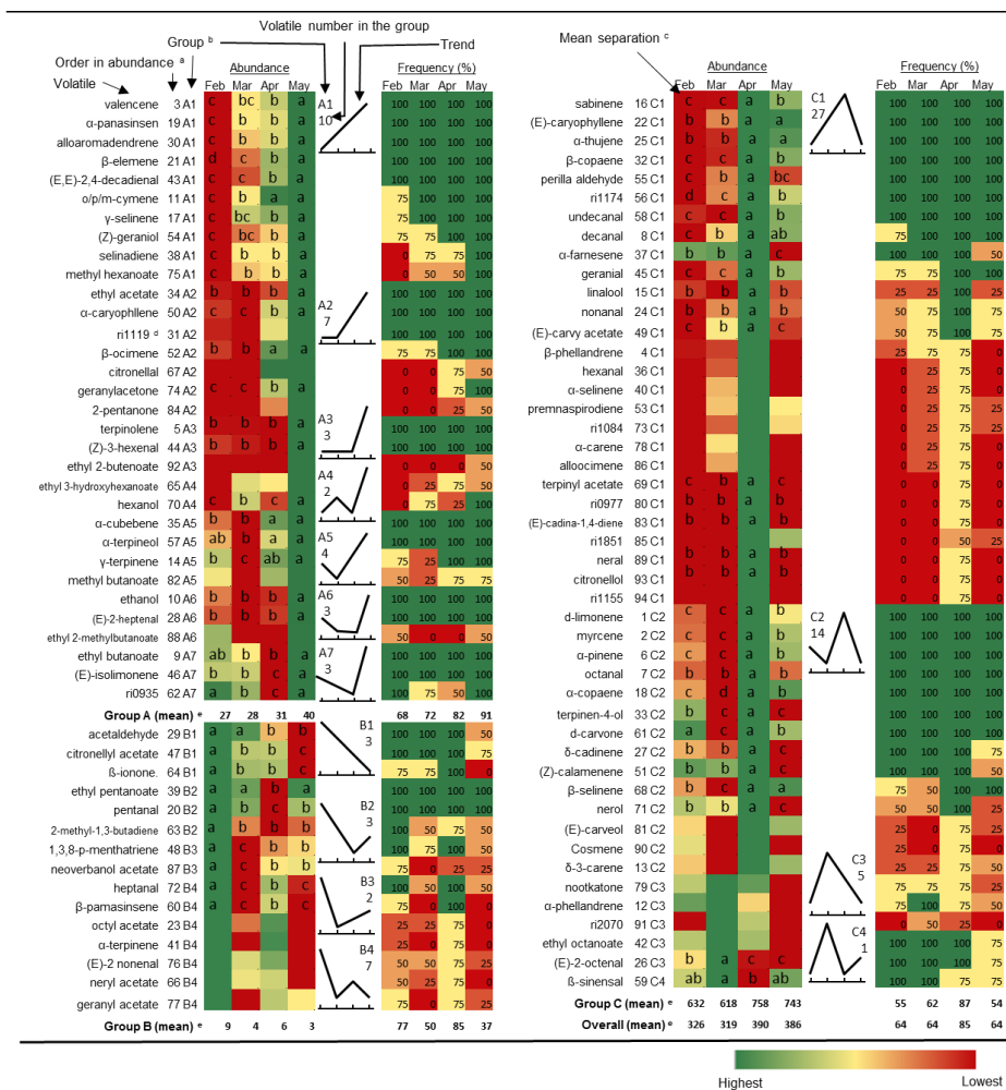
Figure 1. Changes in volatile abundance and frequency of detection in “Valencia” orange juice samples harvested from February to May 2012 ( n = 4 ). a order in abundance listed by average peak size (total ion current) from high to low in total of 94 peaks; b groups: A-increase; B-decrease; C-peak with sub-groups in numbers; c the same letter within the same row (compound) represents no significant different at 0.05 level; d unknown compound with the retention indices (ri + a 4 digital number); e Average abundance ( \times 10^7 total ion current) and frequency of detection (%).
