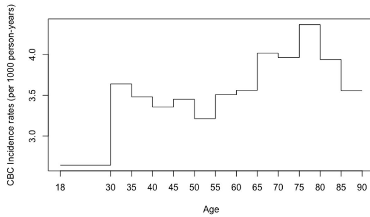
Figure 1. Age-specific composite incidence rates of CBC estimated using SEER data. Age on the horizontal axis can be interpreted as age at counseling.
