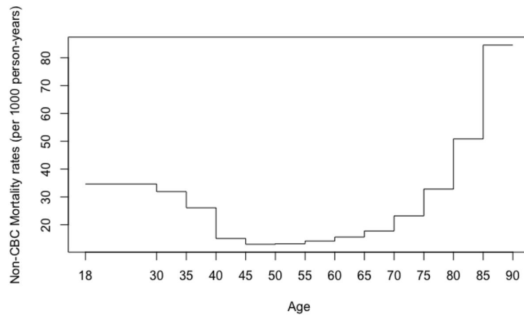
Figure 2. Age-specific mortal hazard rates from non-CBC causes estimated using SEER data. Age on the horizontal axis can be interpreted as age at counseling.
