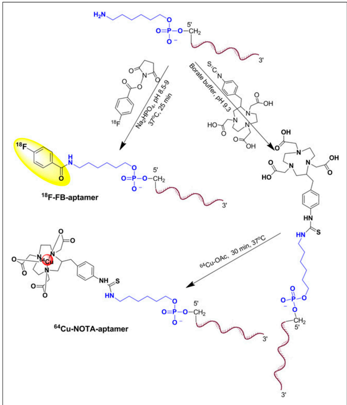
FIGURE 2. ^{18}\text{F} and ^{64}\text{Cu} aptamer labeling routes.
