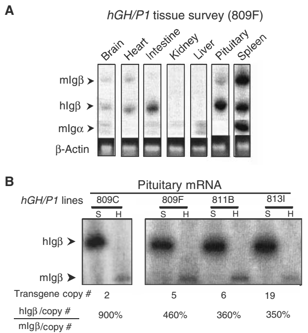
Figure 2 Igβ is transcribed from the hGH/PI transgene in the mouse pituitary. (A) Tissue survey of hGH/PI transgenic mice revealed abundant hIgβ mRNA in the pituitary. A co-RT/PCR endonuclease cleavage assay was used to analyze the tissue specificity of hIgβ expression in a representative hGH/PI transgenic mouse line (line 809F). The RT/PCR assay was identical to Figure 1B with the exception that the 3' primer is 32 P-end labeled. The figure shows the PCR products digested with Sfi I; the larger band (336 bp) corresponds to mIgβ and the smaller (250 bp) to hIgβ (labeled arrows). A separate RT/PCR of mIgα mRNA was carried out to monitor B-lymphocyte contamination in each tissue. The levels of hIgβ , mIgβ , and mIgα are shown relative to a β-actin mRNA loading control (ethidium bromide-stained gel). (B) Pituitary expression of hIgβ mRNA from the hGH/PI transgene was copy number dependent. Pituitaries from four hGH/PI transgenic mouse lines were assayed by RT/PCR for hIgβ mRNA. The level of hIgβ mRNA was normalized to endogenous mouse pituitary Igβ mRNA and this value is shown as a percentage below each pair of lanes after correction for gene copy number.
