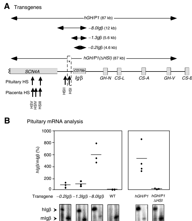
Figure 5 hlgβ expression in the transgenic pituitary is dependent on the hGH LCR. (A) Transgene constructs. A map of the hGH gene cluster is shown. Horizontal arrows above the map indicate the extent of each transgene. The sizes of the constructs are indicated in parentheses and the designation of each construct indicates the extent of sequences 5' from the hlgβ gene promoter. Note that hGH/P1 and -8.0Igβ transgenes include HSI whereas this determinant is excluded from the -0.2Igβ and -1.3Igβ transgenes. In hGH/P1(ΔHSI) , a 99 bp segment (dashed box), corresponding to the critical core elements of HSI, has been deleted from the hGH/P1 transgene (Ho 2002). (B) HSI of the hGH LCR is a critical determinant of pituitary hlgβ expression. The ratios of pituitary hlgβ to mIlgβ mRNAs in the series of hlgβ transgenic mouse lines (A) are shown. Mice from F1 or later generations and from at least three independent lines (dots) were analyzed (X-axis). The hlgβ to mIlgβ mRNA ratios in each transgenic pituitary were plotted on the Y-axis as a percentage. The horizontal lines represent the mean values for each construct in the three or more lines analyzed. Representative co-RT/PCR endonuclease cleavage assays corresponding to each construct are shown below the graph. Wild-type mouse (WT) pituitary RNA was used as negative control. Expression ratios were corrected for transgene copy number.
