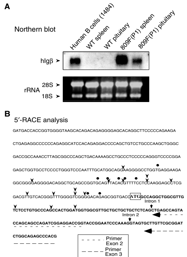
Figure 3 Structural comparison of hIgβ mRNAs in the transgenic pituitary and B cells. (A) Northern blot analysis. Total RNAs from a human B-cell line (1484), from wild-type (WT) mouse lymphocytes (spleen) and pituitary, and lymphocytes (spleen) and pituitary of hGH/PI transgenic mouse line 809F were hybridized with a [ 32 P] labeled hIgβ cDNA probe. The gel was stained with ethidium bromide to visualize 18S and 28S rRNAs as loading control. The hIgβ mRNA hybridizing bands comigrated in all tissues. No additional bands were detected. The absence of signal in the lanes containing WT lymphocytes and pituitary RNA confirmed the species specificity of the hIgβ probe. (B) Mapping the 5' terminus of pituitary and B-cell Igβ mRNAs. The sequence of the hIgβ 5'-flanking region and 5'-terminal transcribed region are shown; the translation start site, ATG , is boxed. The 5' termini of the transcribed mRNAs in B cells and transgenic pituitary were determined by 5' RACE. The arrowheads indicate transcription start sites of hIgβ in the hGH/PI transgenic mouse pituitary mRNA population. The dots indicate the hIgβ start sites in human B-cell line 1484. The figure also indicates the locations of the primers used for the 5'-RACE assay (dashed arrows) and the positions of introns 1 and 2.
