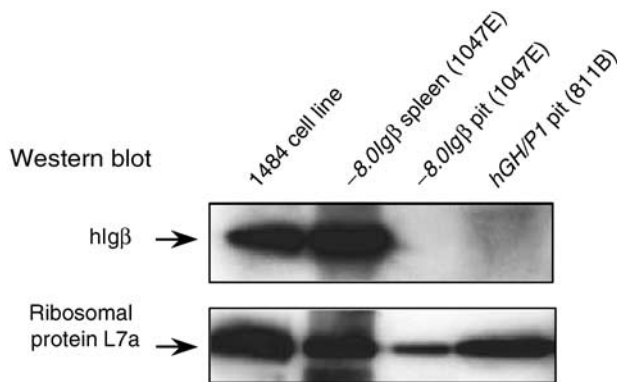
Figure 7 hlgβ protein does not accumulate in hlgβ transgenic mouse pituitaries. Protein extracts from -8.0Ilg\beta and hGH/P1 transgenic pituitaries (lines 1047E and 811B, respectively), human B-cell line 1484, and a -8.0Ilg\beta transgenic spleen (line 1047E) were studied by Western analysis. The top panel was incubated with an antibody to hlgβ and the bottom panel with an antibody to ribosomal protein L7a. Both panels were then developed with secondary antibodies and signals detected by enhanced chemiluminescence. The positions of hlgβ and the ribosomal protein L7 are indicated.
