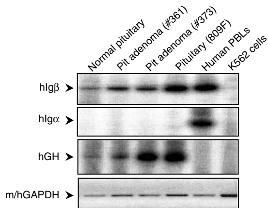
Figure 4 hlgβ mRNA is expressed in human pituitaries. (Top panel) A normal human pituitary and two human pituitary adenomas (#361 and #373) were evaluated for hlgβ mRNA by RT/PCR using 32 P-labeled RT-PCR primers. Positive controls were human peripheral blood lymphocytes (PBLs), hGH/P1 transgenic pituitary (809F line), and the negative control was the human erythroid cell line K562. (Second panel) Igα was monitored by RT/PCR with labeled primers. (Third panel) hGH RT/PCR with labeled primers identified the human and transgenic mouse pituitaries. (Bottom panel) Detection of m/hGAPDH by RT-PCR represented the loading control (ethidium bromide-stained products). All RT/PCR reactions were assayed in the linear range of amplification.
