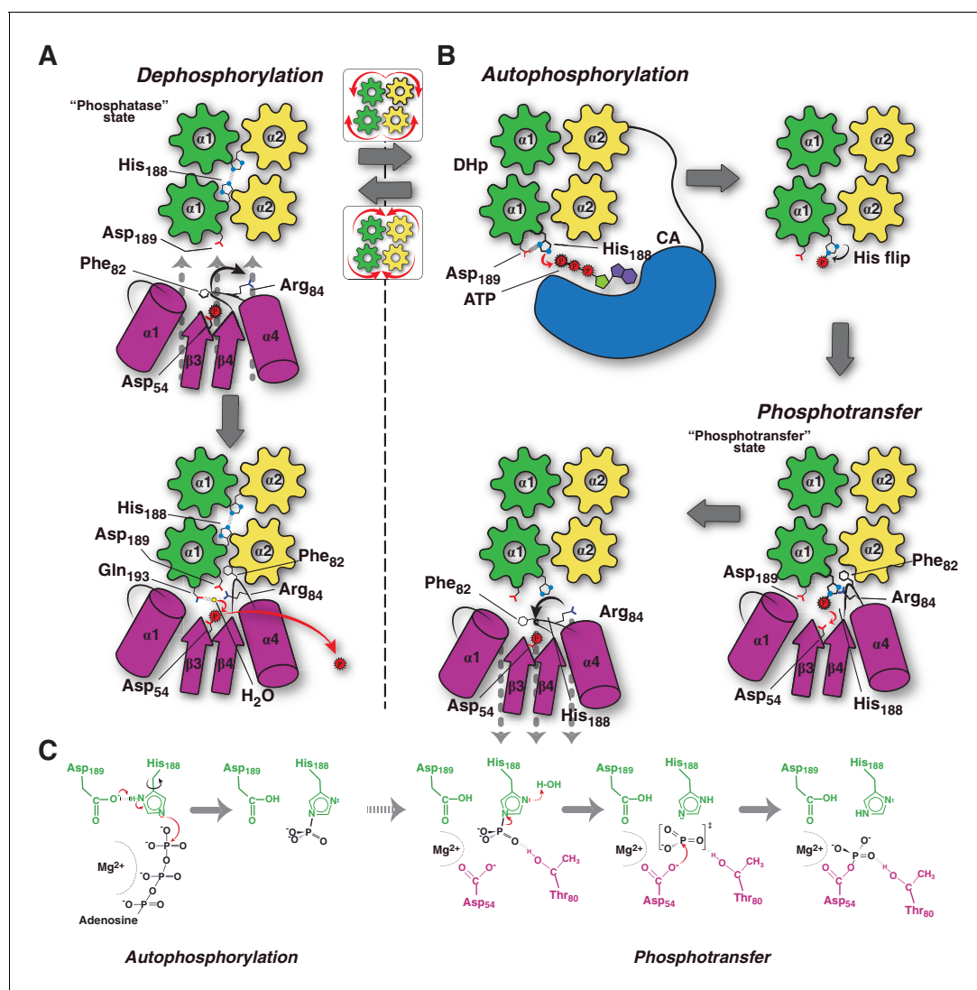
Figure 6. Conceptual model of TCS unidirectional signaling. (A) P~DesR dephosphorylation catalysis is favored by the opening of the RR phosphorylation lid, via Phe 82 (RR) insertion into an HK hydrophobic pocket, and an ionic interaction between Asp 189 (HK) and Arg 84 (RR). The Phe 82 (RR) movement allows for entry of a nucleophilic water (yellow sphere) positioned by Gln 193 (HK). In the phosphatase state the phosphorylatable His 188 (HK) is buried within the DHp domain core, avoiding autophosphorylation and phosphoryl back-transfer reactions. (B) Signal-mediated pathway activation triggers the cogwheel rotation of the HK DHp \alpha -helices, via coiled-coil disruption. The His 188 (HK) becomes exposed to the solvent, CA domains are released, and autophosphorylation thus enabled. Binding to unphosphorylated RR positions the P~His 188 (HK) into a suitable orientation for phosphoryl-transfer to occur through a loose (dissociative) nucleophilic substitution. Movement of Thr 80 (RR) is coupled with phosphoryl group migration, triggering RR's phosphate lid closure and P~RR release. (C) Reaction scheme summarizing the autophosphorylation and phosphotransfer reactions. Stabilization of a protonated N \delta 1 tautomer of the reactive histidine, is required in autophosphorylation. In keeping with the imidazole aromaticity, the nucleophilicity of N \epsilon 2 is thus finely regulated, allowing for phospho-acceptor/donor roles of the His.
