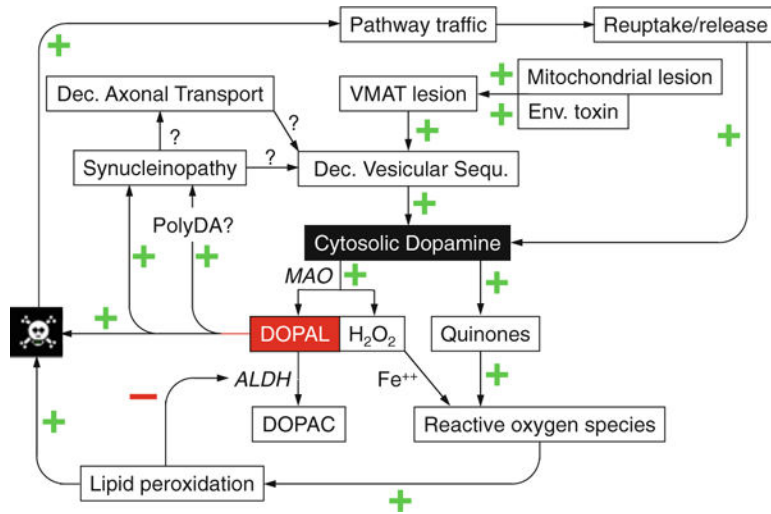
Fig. 3. Overview of pathogenetic mechanisms in catecholaminergic neurons. Central to the vulnerability of these neurons are ongoing vesicular leakage and toxicity of cytosolic catecholamines such as dopamine, via spontaneous auto-oxidation and oxidation catalyzed by monoamine oxidase ( MAO ) to form dihydroxyphenylacetaldehyde ( DOPAL ). DOPAL is detoxified by aldehyde dehydrogenase ( ALDH ) to form dihydroxyphenylacetic acid ( DOPAC ). Other abbreviations: Dec decreased, Env environmental, PolyDA polydopamine, VMAT vesicular monoamine transporter
