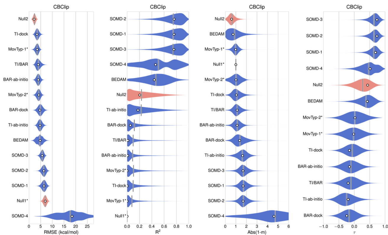
Fig. 4. CBCLIP submissions ranked based on the original values of absolute error metrics ( white circles ), which were computed from reported binding affinities without resampling or considering any uncertainty sources. The violin plot describes the shape of the sampling distribution for each set of predictions when bootstrapping 100,000 samples with replacement, and the vertical bar represents the mean of the distribution. Two null models are shown in red. The computational uncertainties are absent in Null1 model, MovTyp-1 and MoveTyp-2 predictions
