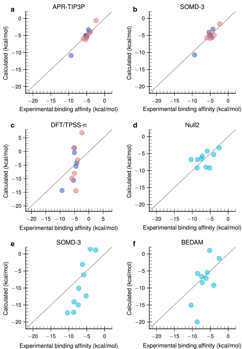
Fig. 5. Combined OAH/OAMe predictions with MSE offsets using a APR-TIP3P, b SOMD-3, and c DFT/TPSS-n method. CBClip predictions without MSE offset using d the Null2 model, e SOMD-3, and f BEDAM method. Purple dots OAH, red dots OAMe, cyan dots CBClip, solid black line of identity
