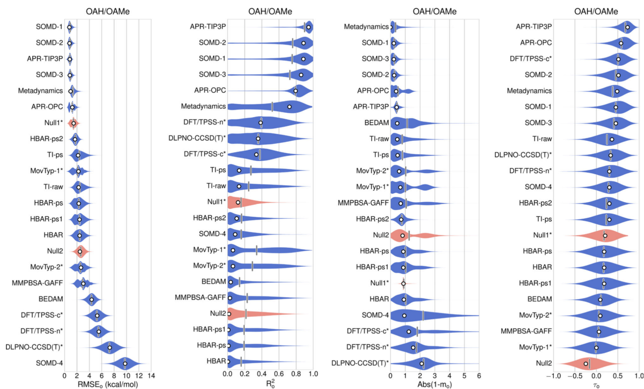
Fig. 3. OAH/OAMe submissions ranked based on the original values of offset error metrics ( white circles ), which were computed from reported binding affinities without resampling or considering any uncertainty sources. The violin plot describes the shape of the sampling distribution for each set of predictions when bootstrapping 100,000 samples with replacement, and the vertical bar represents the mean of the distribution. The computational uncertainties are absent in Null1 model, MovTyp-1, MoveTyp-2 DFT/TPSS-n, DFT/TPSS-C and DLPNO-CCSD(T) predictions. Two null models are shown in red
