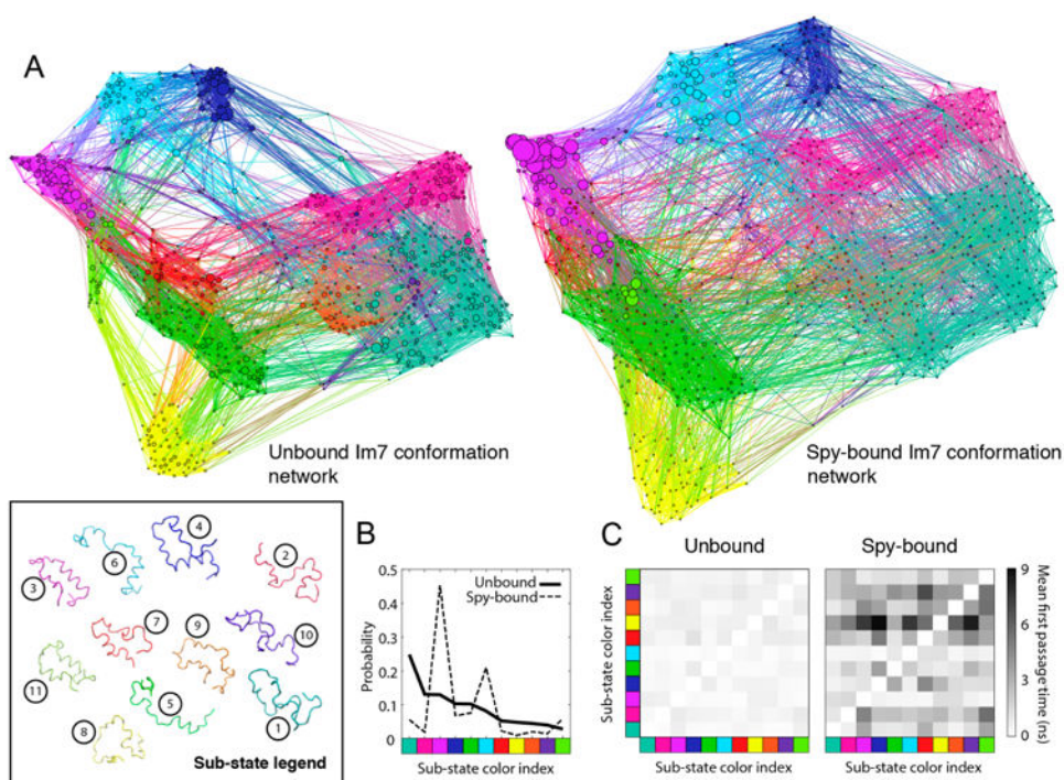
Figure 5. Network and kinetic analysis of Spy-Im 7 6-45 simulations. (A) Conformation-space networks are shown for the unbound and bound ensembles of Im 7 6-45 . The nodes in each network correspond to a particular Im 7 6-45 conformation, and the links between nodes indicate a transition between conformations during simulation. Node size is proportional to the population of a conformation in the ensemble, and the colors denote the substate to which a conformation belongs. The box at the bottom left shows a representative conformation for each of the substates, which are displayed using the same colors as in the networks. The numbers adjacent to each conformation show the index for each substate. (B) Populations of each substate in the bound and unbound ensembles. The indices for the substates are chosen as a ranking for the population in the unbound ensemble: substate 1 has the highest weight and substate 11 has the lowest. Reweighting of the substate population indicates that Im 7 6-45 gains structure upon binding Spy. The axes labels show the color index of the substates, which are ordered according to their indices. (C) The mean first passage time for transitions between substates is shown using a heat map, with black indicating a slow transition and white indicating a fast transition. These data indicate that transitions between different Im 7 6-45 substates are slowed down when bound to Spy.
