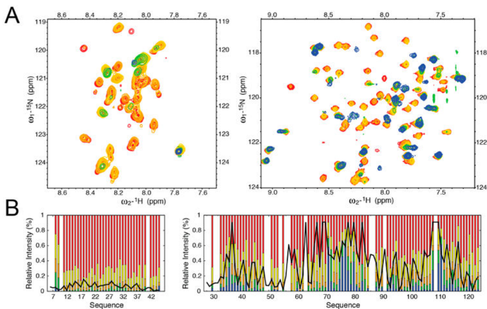
Figure 2. NMR titration of the Spy–Im7 6–45 interaction. (A) 15 N HSQC spectra are shown for protein ratios of 0 (red), 0.1 (yellow), 0.2 (orange), 0.3 (green), and 0.4 (blue) when unlabeled Spy was added to labeled Im7 6–45 (left) and unlabeled Im7 6–45 was added to labeled Spy (right). Addition of Spy results in the significant loss of intensity for several peaks in Im7 6–45 , precluding the possibility of a direct characterization of chaperone–substrate interactions by NMR alone. (B) Comparison of changes in NMR signal intensities from titration experiments to the chaperone and substrate interaction patterns observed in the binding simulations. Relative intensities, compared to the free forms, of the resonances observed in Im7 6–45 (left) and Spy (right) upon titration. Color-coding is the same as in (A). Black lines correspond to the pseudoenergy of contact between Spy and Im7 6–45 (arbitrary units) obtained from coarse-grained simulation of the complex using the optimized force field. Low values indicate favorable regions for chaperone–substrate interactions.
