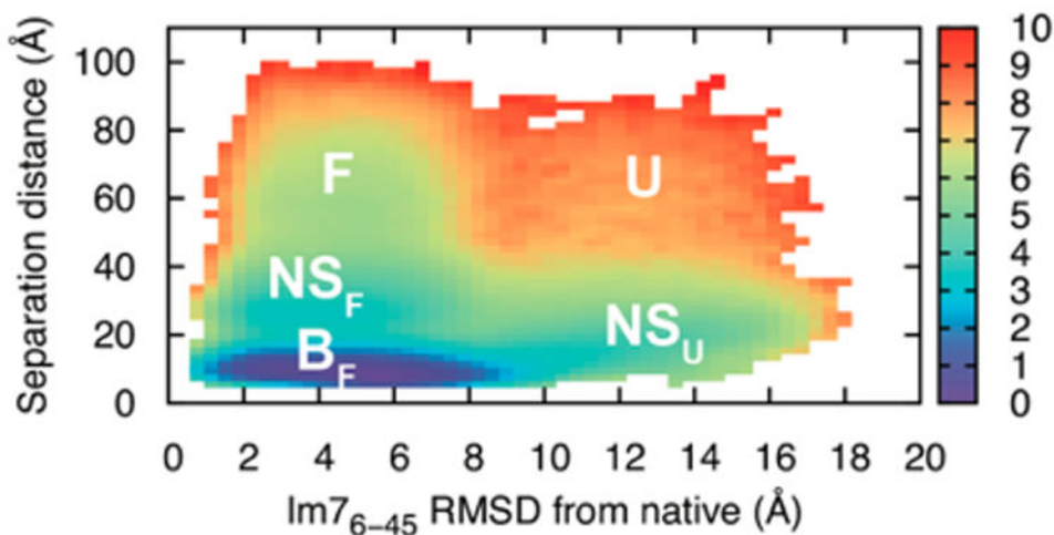
Figure 6. Spy-Im7 6-45 binding mechanism. A free energy surface of the Spy-Im7 6-45 separation distance and the C \alpha -RMSD of Im7 6-45 to the equivalent segment in the crystal structure of full-length, native-state Im7. The separation distance is defined as the distance between the centers of mass of Spy and Im7 6-45 . The labels signify different conformational states of the Im7 6-45 substrate in the presence of the Spy chaperone: B F (bound and largely folded), NS F (nonspecific complex and folded), NS U (nonspecific complex and unfolded), F (unbound and well-folded), and U (unbound and unfolded). The surface is computed at the simulation temperature of 300 K and the colorbar denotes the free energy in units of kcal/mol. The free energy is normalized by the volume of a spherical shell with a radius corresponding to a given distance.
