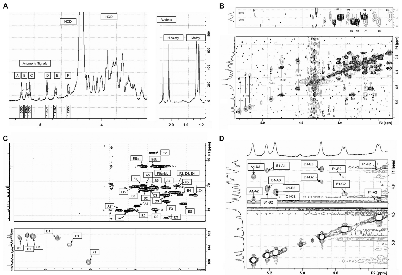
FIG 2 NMR analysis of the EPS isolated from Lactobacillus paracasei DG. (A) Selected regions of the ^1\text{H} -NMR spectrum of DG-EPS recorded at 70^\circ\text{C} in \text{D}_2\text{O} using acetone as an internal standard. Anomeric ( \text{H}-1 ) resonances are labeled A to F in order of decreasing chemical shift. (B) Selected regions of overlaid COSY (black contours) and TOCSY (gray contours) spectra for DG-EPS recorded at 70^\circ\text{C} . Top, ^{13}\text{C} -methyl region; bottom, ^{13}\text{C} region for anomeric and ring protons. The letters A to F designate individual sugars, and numbers 1 to 6 indicate the C/H ring position. (C) Selected regions of the HSQC spectrum of DG-EPS. (Top) Locations of the individual rings and H6 protons and carbons; (bottom) locations of the anomeric protons and carbons. The spectrum was recorded in \text{D}_2\text{O} at 70^\circ\text{C} . (D) Anomeric region of a ROESY spectrum recorded for DG-EPS. Inter- and intraresidue NOEs from the anomeric hydrogens to ring protons are individually labeled.
