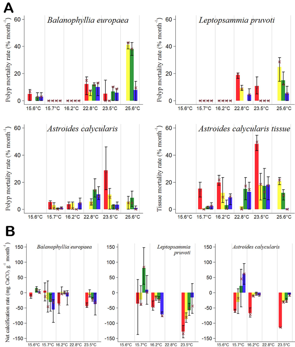
Figure 1. Plots of the values of mortality and net calcification rates for each average \text{pH}_{\text{TS}} value of each site and for each transplantation period for the three coral species. The acidity is indicated by the different colours: red (Site 4 - \text{pH}_{\text{TS}} 7.40), yellow (Site 3 - \text{pH}_{\text{TS}} 7.74), green (Site 2 - \text{pH}_{\text{TS}} 7.87), blue (Site 1 - \text{pH}_{\text{TS}} 8.07). Each transplantation period is denoted by the average seawater temperature. Average values = height of the histogram bars; median = cross, 10–90 percentiles intervals = error bars. Empty bins in the histograms indicate missing data due to storms that swept away the experiments. (A) Mortality rates (% month -1 ). Polyp mortality rate for B. europaea , L. pruvoti , and A. calycularis and coenosarc-polyp tissue mortality for the latter. For B. europaea and L. pruvoti at 15.7°C and 16.2°C and for the latter also at 23.5°C the cross symbols indicate zero mortality. (B) Net calcification rates (mg CaCO 3 g -1 month -1 ) for B. europaea , L. pruvoti , and A. calycularis .
