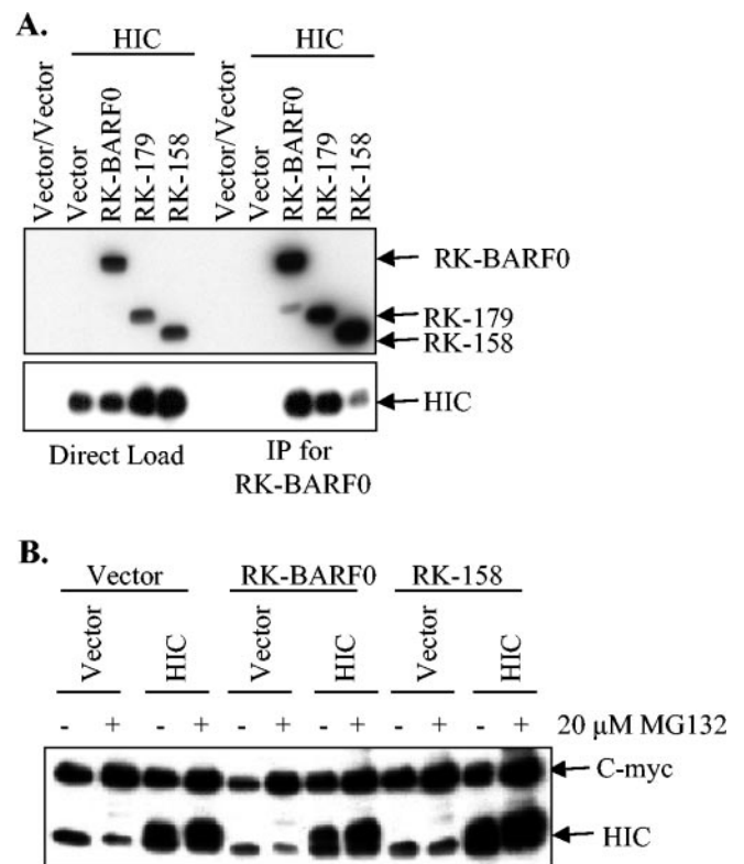
FIG. 3. RK-BARF0 binds HIC but does not induce proteasome-dependent degradation. (A) Flag- and His6-tagged RK-BARF0, RK-179, and RK-158 were transiently transfected into H1299 cells with myc-tagged HIC. Lysates were directly loaded onto an SDS-PAGE gel (left panel) or immunoprecipitated (IP) with \alpha -Flag (right panel). RK-BARF0 was detected with \alpha -His6, and HIC was detected with \alpha -cMyc. (B) RK-BARF0 and RK-158 were transiently transfected into H1299 cells with HIC and were treated with 20 \mu M MG132 to examine degradation of HIC. HIC was detected with \alpha -cMyc.
