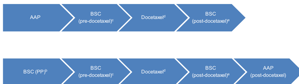
Fig. 1 Visual representation of the DES model (see Figs. 5.1 and 5.2 from the ERG report [3] for more details). DES discrete event simulation, AAP abiraterone acetate in combination with prednisone/prednisolone, BSC best supportive care, PP placebo plus prednisone/prednisolone, ERG Evidence Review Group, ECOG Eastern Cooperative Oncology Group, PS performance score. a Patients could die in all stages of the model, except during AAP, BSC (PP), and post-docetaxel treatment. If patients die, they firstly go through the ‘BSC before death’ phase involving palliative care, until death. This consists of the ‘end-of-life’ phase where patients are near death and will not receive additional active treatments that may impact survival, but instead are managed for their pain or other symptoms. b BSC (PP) involves active monitoring without active treatments that impact survival (patients are still receiving treatments that palliate symptoms
