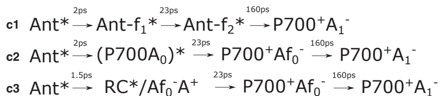
FIGURE 13 Possible contributors to the compartments in the FRL-PSI sequential model results for 670 nm and 700 nm excitation. Abbreviations are the same as in Fig. 1, with Ant- f and Af_0^- denoting Chl f pigments in the antenna and replacing A_0 correspondingly. See text for more details.
