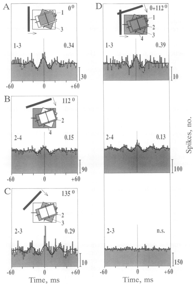
FIG. 1. Conflicting stimuli alter the cross-columnar interaction. We recorded simultaneously from four different sites separated by 400\ \mu\text{m} . Cells at recording sites 1 and 3 preferred stimulus orientations near vertical. In contrast, cells at sites 2 and 4 had orientation preferences near horizontal (indicated by the thick line drawn across each receptive field in A–D). Stimulation with single light bars of 0^\circ (A), 112^\circ (B), and 135^\circ (C) orientation yielded a synchronization between all responding sites (hatched receptive fields). (D) With combined presentation of both 0^\circ and 112^\circ light bars, responses were synchronized between sites 1 and 3 and between sites 2 and 4. However, no significant (n.s.) synchronization occurred between these pairs—e.g., between responses 2 and 3. The cross-correlograms between sites 1 and 2, sites 1 and 4, and sites 3 and 4 were also flat (data not shown). The graph superimposed on each of the correlograms represents the Gabor function used to assess strength of the modulation. The number at the upper right of each correlogram indicates relative modulation amplitude. Note that, for both pairs 1, 3 and 2, 4, relative modulation amplitude was undiminished with the conflicting stimuli. Scale bars indicate number of spikes. (This figure is adapted, with modification, from ref. 21.)
