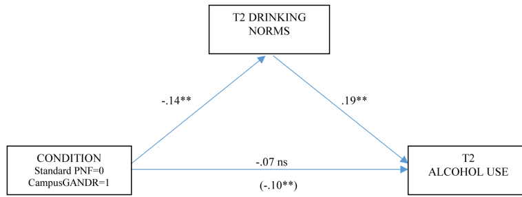
Figure 5. Supported mediation model with unstandardized regression coefficients for all paths including the (total effect) of x on y . * p < .05 ; ** p < .01 .
