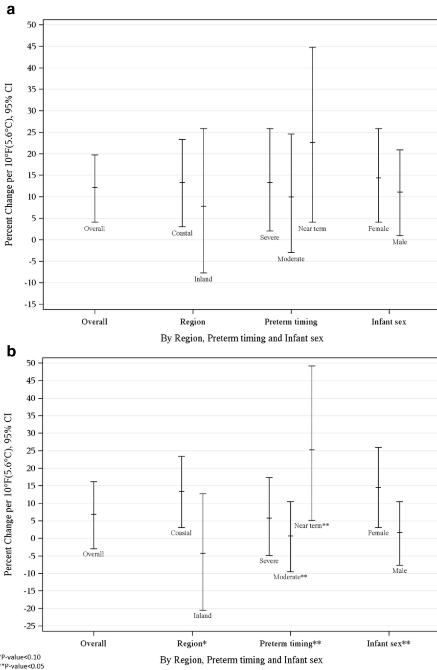
Fig. 3 a Estimated Percent Change Associated with a 10 °F(5.6 °C) Increase in Weekly Average Apparent Temperature and Spontaneous Preterm Delivery during the Warm Season, Overall and by Region, Preterm Delivery Timing and Infant Sex. b Estimated Percent Change Associated with a 10 °F(5.6 °C) Increase in Weekly Average Apparent Temperature and Spontaneous Preterm Delivery during the Cold Season, Overall and by Region, Preterm Delivery Timing and Infant Sex
