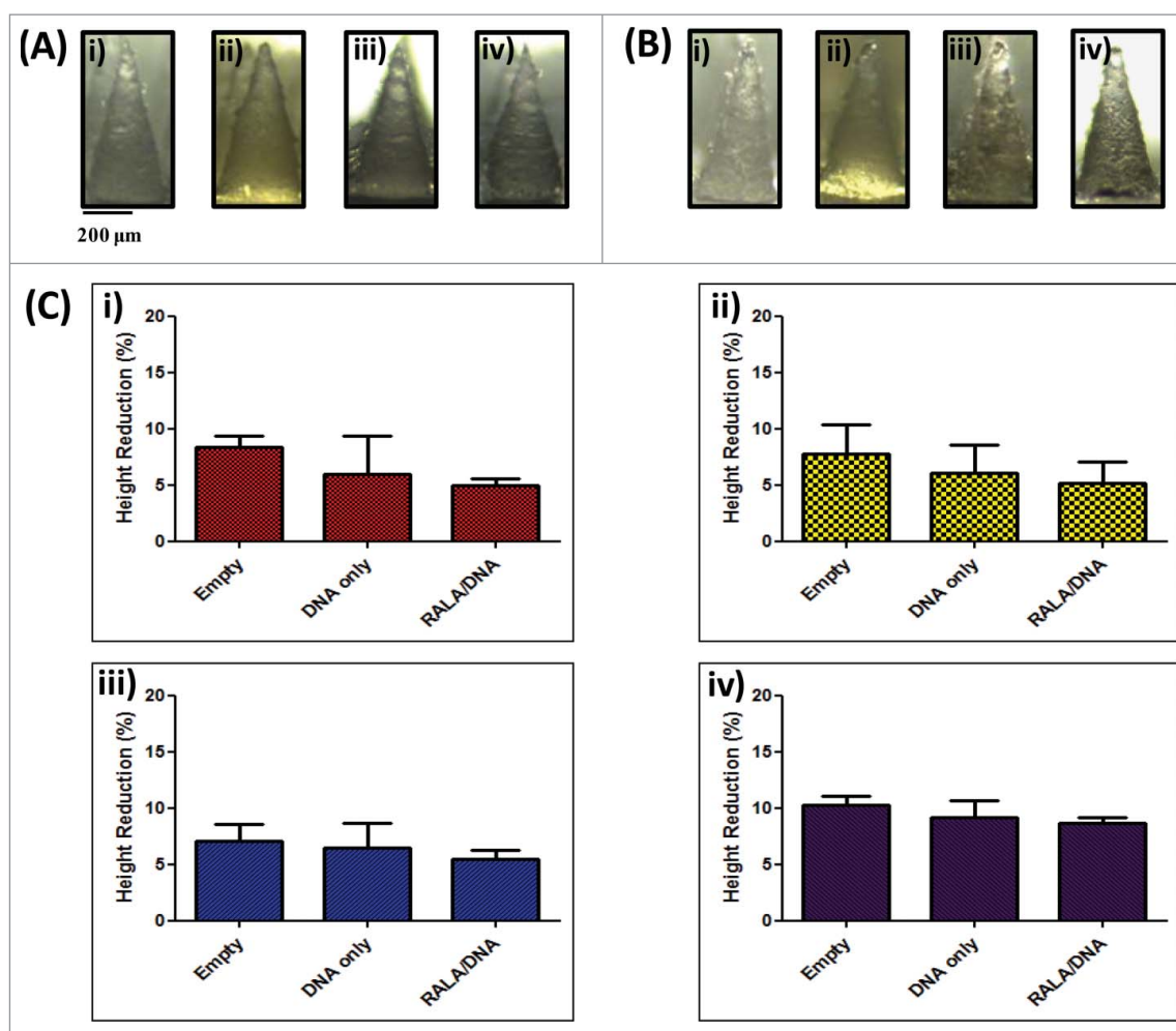
Figure 5. Characterization of dissolvable microneedle arrays loaded with DNA (N:(P)0) and RALA/DNA nanoparticles (N:(P)10). (A) Digital microscope images of microneedles formulated from i) 360 kDa PVP, ii) 58 kDa PVP, iii) 13–23 kDa PVA and iv) 9–10 kDa PVA loaded with RALA/DNA nanoparticles (N:P 10) prior to and (B) following 45 N axial compression; (C) Percentage height reduction of i) 360 kDa PVP, ii) 58 kDa PVP, iii) 13–23 kDa PVA and iv) 9–10 kDa PVA arrays, unloaded or loaded with DNA only (N:P 0) or RALA/DNA nanoparticles (N:P 10) following 45 N compression (means + SEM, N = 3).
