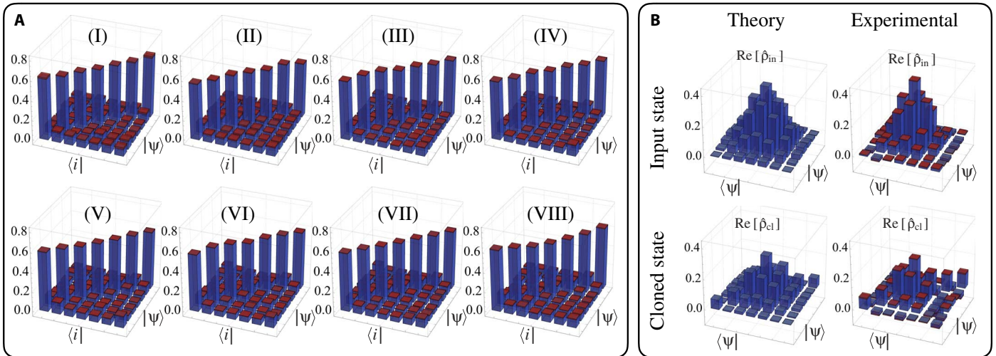
Fig. 3. Cloning fidelities for various MUBs and cloning of Gaussian states in dimension d = 7 . (A) Probability \mathcal{P}(|j\rangle, |\psi\rangle) of detection of an output cloned state |j\rangle given an input state |\psi\rangle , where |j\rangle and |\psi\rangle belong to a specific MUB. This set of measurement is repeated for all d + 1 MUBs (I) to (VIII), in dimension 7. The on-diagonal elements represent the cloning fidelities for each element of a given basis. (B) Theoretical and experimental high-dimensional cloning of a Gaussian state. The cloned fidelity is obtained by calculating the overlap of the reduced density matrix of the cloned state with the input state. The experimental reduced density matrix of the cloned state is obtained by full quantum state tomography. The experimentally reconstructed density matrices of the Gaussian state before and after cloning are shown along with their theoretical counterparts.
