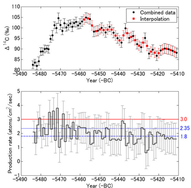
Fig. 3. The ^{14}\text{C} production rate for the period from 5484 BC to 5411 BC using a four-box model. We calculated the production rates in this graph using the steady state as 1.8 atoms per square centimeter per second. The blue dashed line (1.8 atoms per square centimeter per second) marks the production rate of normal solar magnetic activity, the blue dotted line (2.35 atoms per square centimeter per second) is average production rate for the Maunder Minimum, and the red solid line (3.0 atoms per square centimeter per second) is the production rate in the case where the solar modulation parameter becomes zero.
