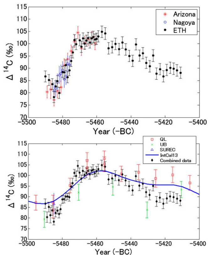
Fig. 1. (Upper) Measured results [ \Delta^{14}\text{C} : defined in Stuiver and Polach (29)] of three series that were measured at different AMS laboratories (Arizona, Nagoya, and ETH). (Lower) Comparison of our combined data (diamonds: bristlecone pine), the original datasets of the IntCal [QL (6), UB (30), and SUREC (31)], and the IntCal13 curve (1). Although the IntCal original data are not consistent with each other, our measured results almost agree with the IntCal13.
