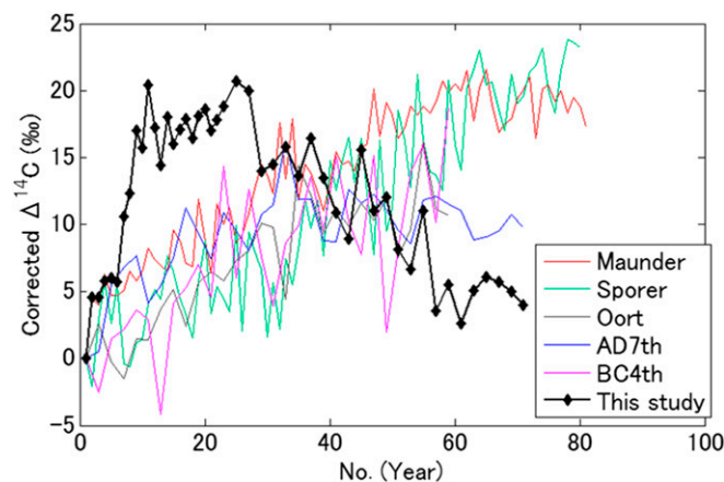
Fig. 2. Comparison of the 5480 BC event with other grand solar minima (6, 20–22). The origin of the coordinates corresponds to the shifted data point of the first year of each grand solar minima (18), and the 5481 BC data point shown in Fig. 1. Further information about the grand solar minima is provided in Table S2.
