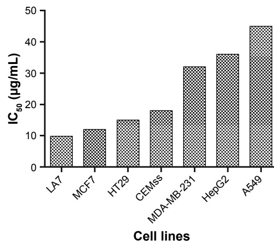
Figure 2 Cytotoxicity effect of KME against different cell lines. Abbreviations: \text{IC}_{50} , half maximal inhibitory concentration; KME, Kelussia odoratissima methanol extract.
