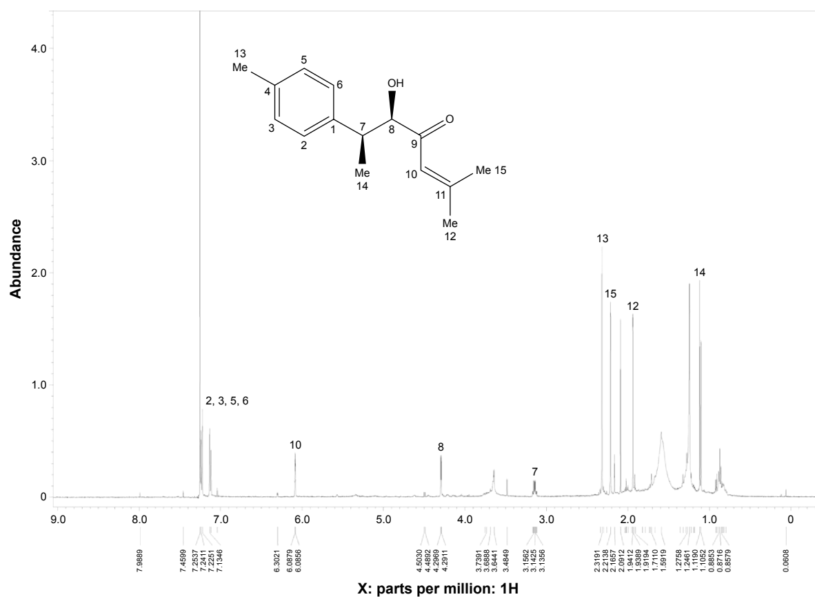
Figure 1 1 H NMR and chemical structures of 8-hydroxy-ar-turmerone. Abbreviation: NMR, nuclear magnetic resonance.
