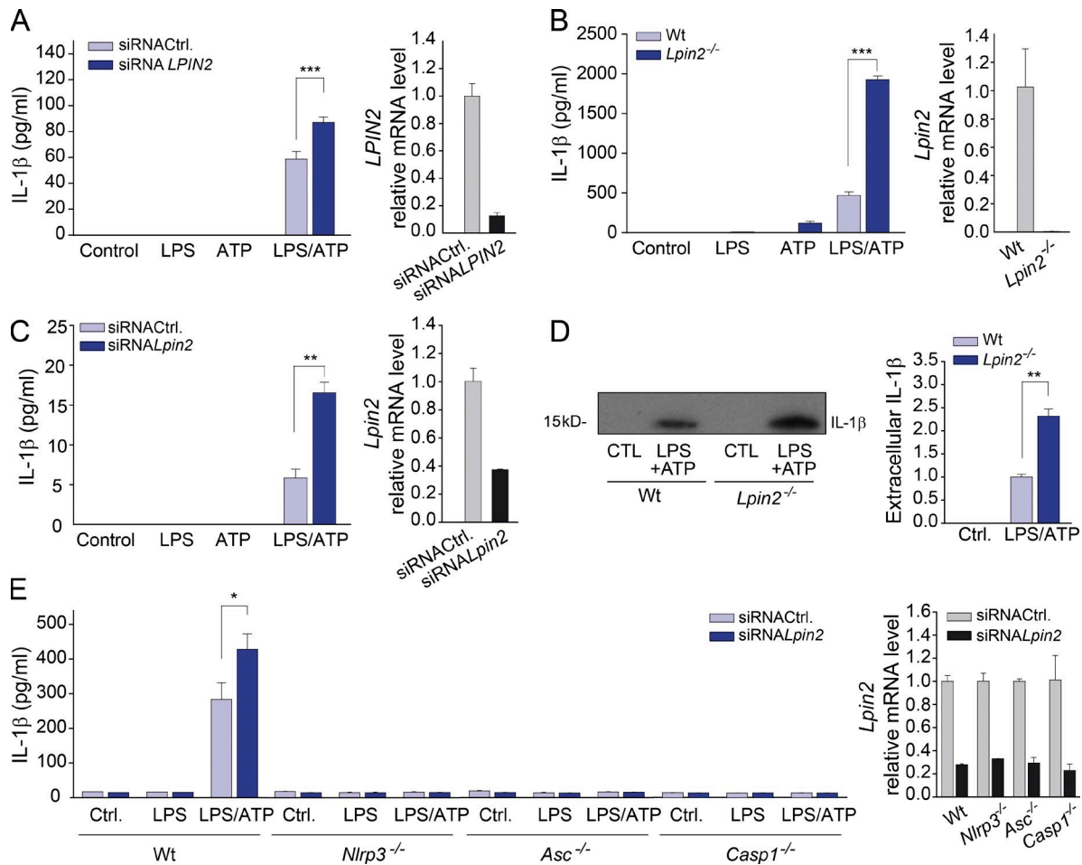
Figure 1. The effect of lipin-2 on IL-1 \beta production by murine and human macrophages. IL-1 \beta presence in supernatants from primary human macrophages (A), BMDMs from WT and Lpin2^{-/-} mice (B and D), or RAW264.7 cells (C) stimulated with 200 ng/ml LPS for 4 h, 2 mM ATP for 40 min, or both, as indicated, were quantified by specific ELISAs. (A–C) Human macrophages and RAW264.7 cells were silenced as described in Materials and methods, using control (siRNACtrl.) and lipin-2-specific siRNAs (siRNA Lpin2 ). (right) Lpin2 mRNA levels at the time of stimulation. (D) BMDMs supernatants were analyzed by immunoblot using specific antibodies against IL-1 \beta . (right) Densitometric quantification of the bands. (E) IL-1 \beta production was analyzed in BMDMs supernatants from WT, Nlrp3^{-/-} , Asc^{-/-} , and Casp1^{-/-} animals treated with a control siRNA (siRNACtrl.) or siRNAs against Lpin2 (siRNA Lpin2 ) for 2 d, and then stimulated as indicated. (right) Level of Lpin2 mRNA after silencing. Data from A–C and E are shown as means \pm SD and are representative of at least three independent experiments made in triplicate. Data from D are representative of at least three independent experiments. *, P < 0.05 ; **, P < 0.01 ; ***, P < 0.001 , Student's t test.
