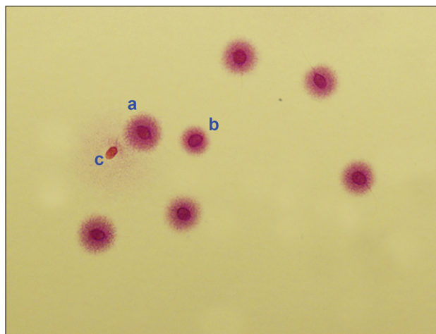
Figure 1: Sperm chromatin dispersion test. (a) A big halo represents no DNA fragmentation, (b) a medium halo represents no DNA fragmentation, and (c) no halo indicates spermatozoa with DNA fragmentation
