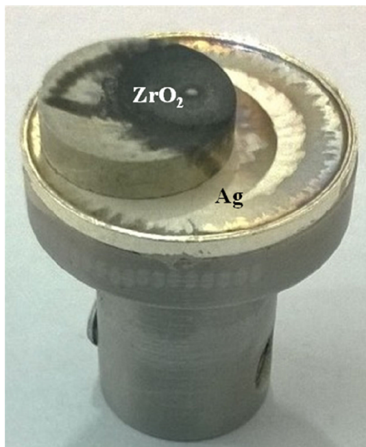
Fig. 1 Target holder consists of Ag and ZrO 2
