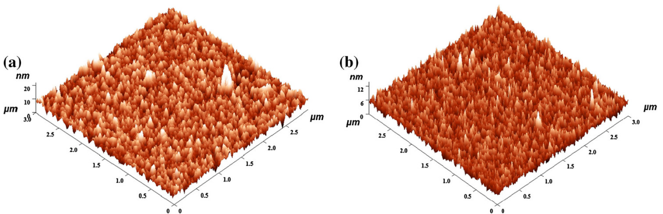
Fig. 4 Three-dimensional (3D) projections of typical AFM images and surface profiles of ZrO_2 (a) and Ag- ZrO_2 composite coatings (b) coated 316L SS from approximately 3 \times 3 \mu\text{m} scanned areas
