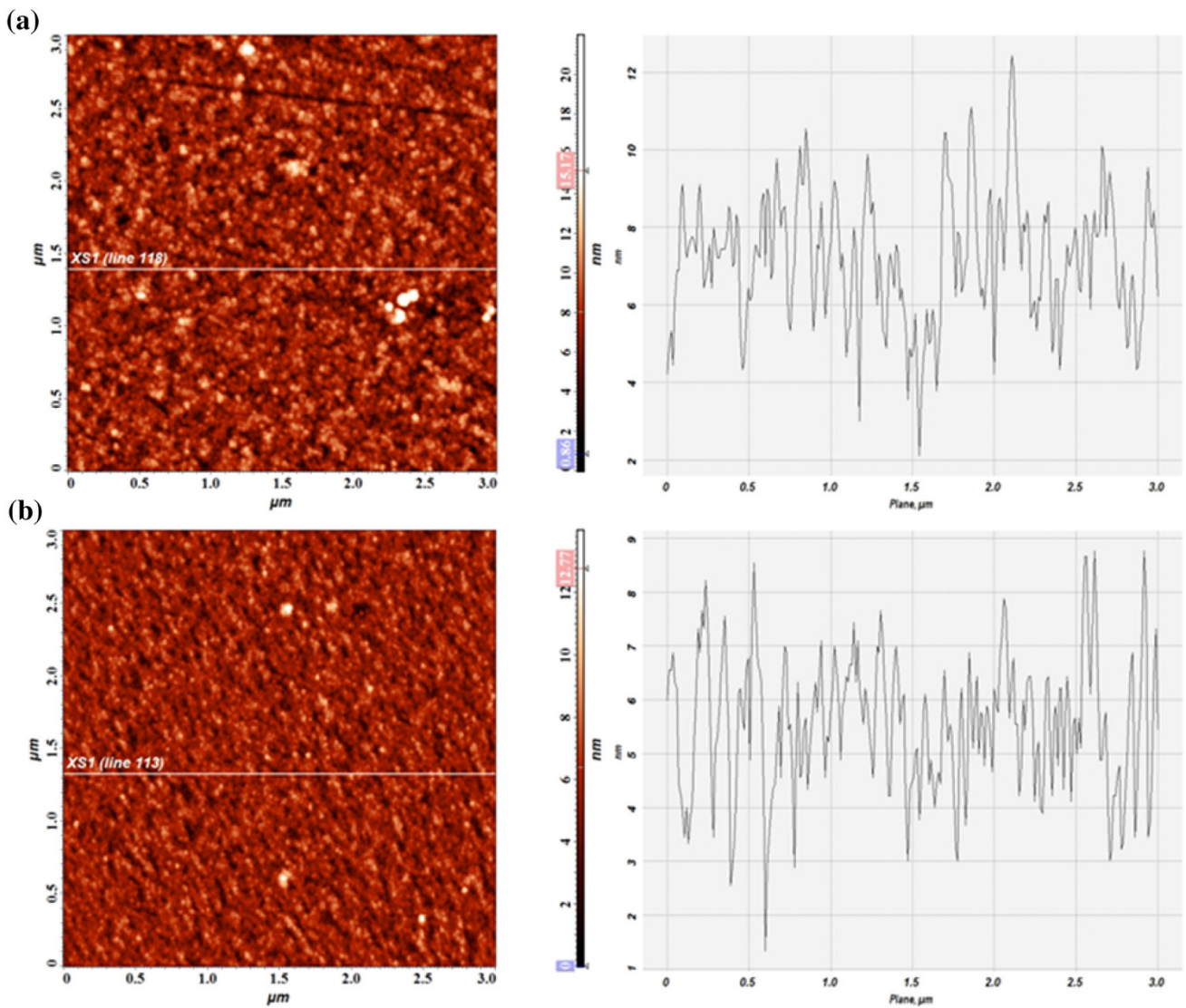
Fig. 3 Two-dimensional (2D) AFM images and surface profiles of ZrO_2 (a) and Ag- ZrO_2 composite coatings (b) coated 316L SS from approximately 3 \times 3 \mu\text{m} scanned areas
