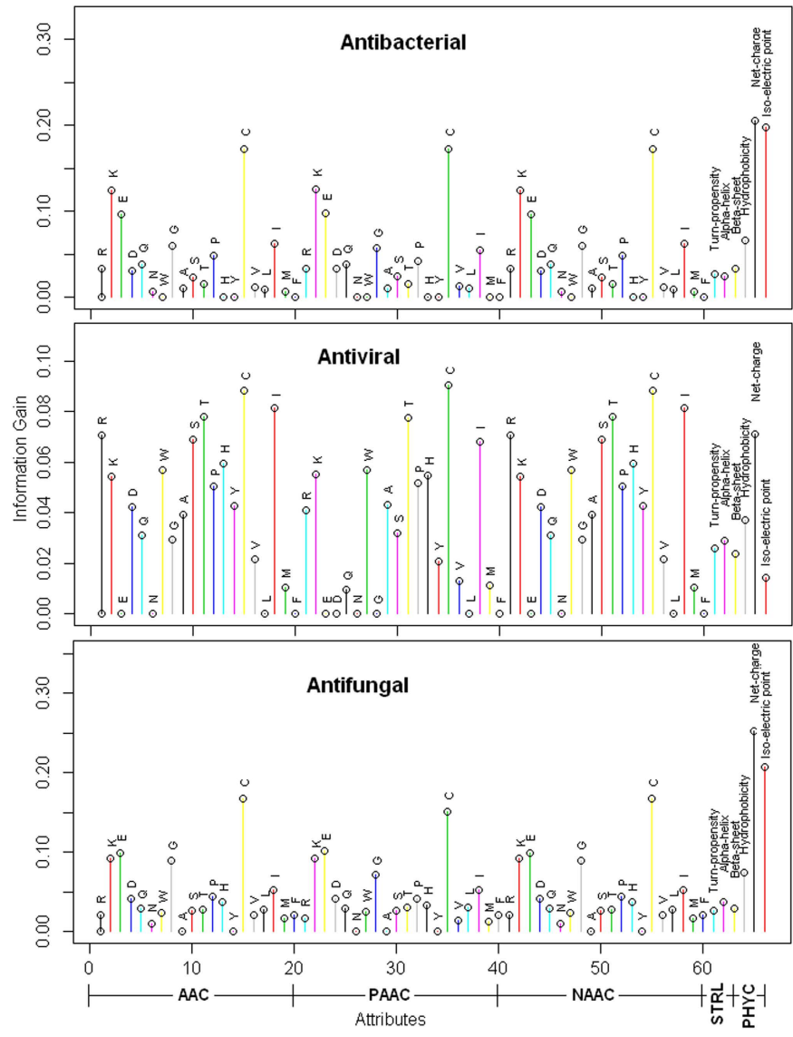
Figure 1. Information gain for all the 66 features [AAC (20) + PAAC (20) + NAAC (20) + PHYC (3) + STRL (3)] in predicting antibacterial, antiviral and antifungal peptides.
