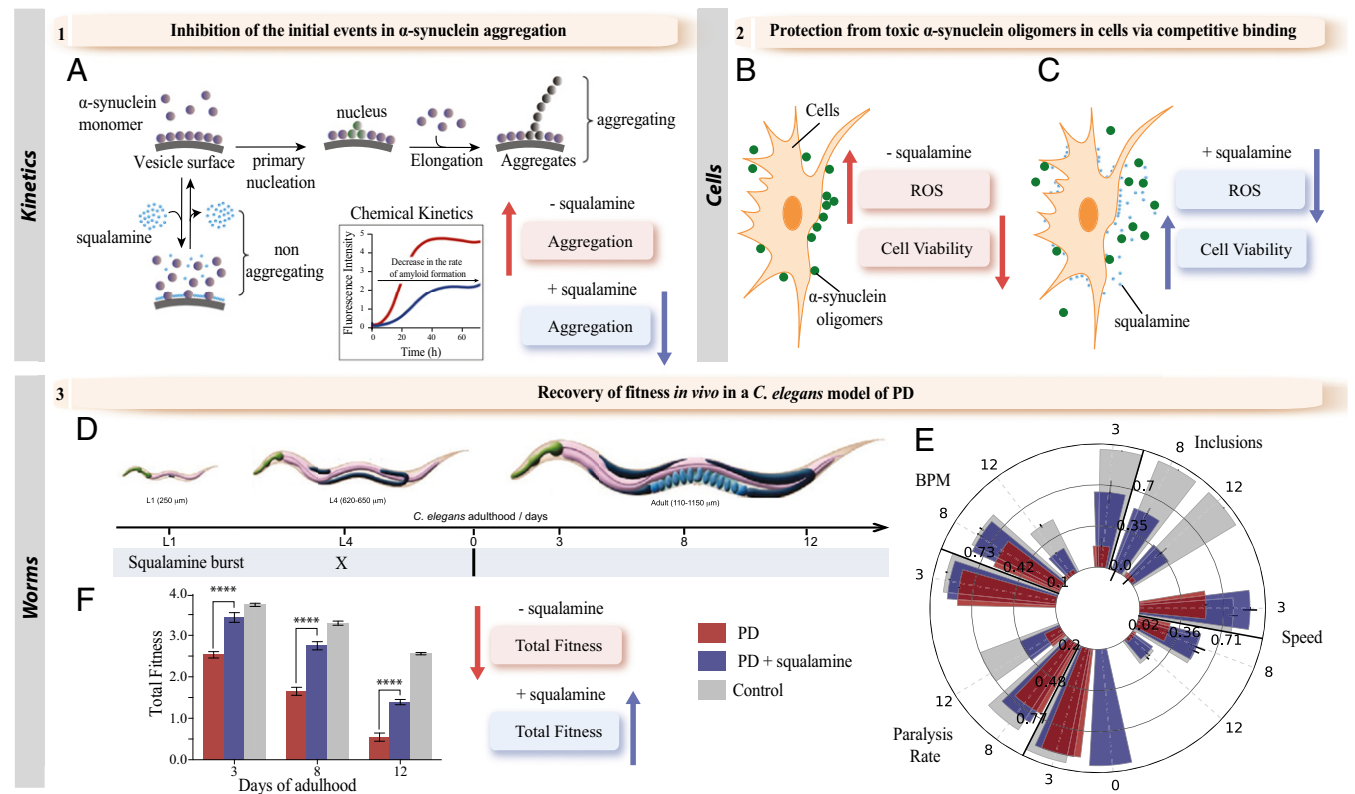
Fig. 6. Schematic illustration of the drug discovery strategy used in this work. (A) We used a wide range of biophysical techniques, including chemical kinetics, to study quantitatively the effects of squalamine on \alpha -synuclein aggregation in vitro and we observed that squalamine affects the binding of \alpha -synuclein to lipid membranes and inhibits the initial events in its aggregation. (B and C) By using the protocols that we recently developed to isolate oligomers of \alpha -synuclein toxic to human cells (23, 24), we have shown that squalamine inhibits dramatically the mitochondrial dysfunction and cellular ROS production induced by the oligomers of \alpha -synuclein (23, 24). (D–F) We further validated our results in vivo by using a well-established C. elegans model of PD (25), and we found that administration of a single dose of squalamine at the larval stage L4 (D) abolishes \alpha -synuclein aggregation and its associated toxicity in vivo over several days (E) and increases the total fitness of the PD worms (F).
