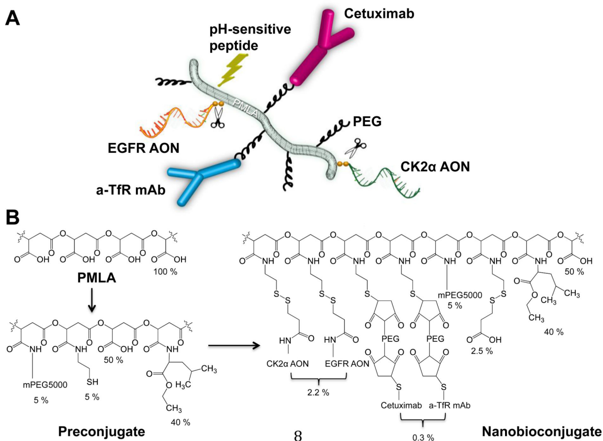
Figure 1. Multifunctional nanobioconjugates used to treat glioblastoma multiforme (GBM). A) Schematic structure of the complete nanobioconjugate showing functional moieties. PMLA - poly( \beta -L-malic acid), EGFR - epidermal growth factor receptor, AON - antisense oligonucleotide, PEG - polyethylene glycol, a-TfR - anti-mouse transferrin receptor to cross the BBB by transcytosis, mAb - monoclonal antibody, Cetuximab - anti-human EGFR antibody to target tumor cells, CK2 \alpha - catalytic \alpha subunit of protein kinase CK2. Scissors denote AON S-S sites of cleavage from PMLA by cytoplasmic glutathione. B) Chemical synthesis of nanobioconjugate from PMLA through the preconjugate stage to the complete nanobioconjugate. Percentage contents of functional units are shown. mPEG - methoxy polyethylene glycol.
