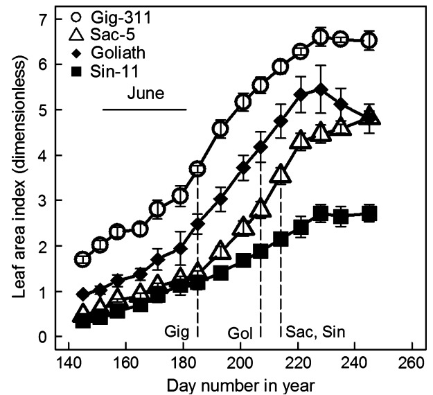
Fig. 4 The mean LAIs across the replicate trial plots for the four genotypes (in 2011) vs. day number in the year. The error bars are plus-and-minus one standard error of the means. The vertical lines show when the canopies first intercepted 90% or more of the incident PAR based on the LAIs and the fitted k values. The horizontal bar indicates June which has the peak in the annual PAR levels.
