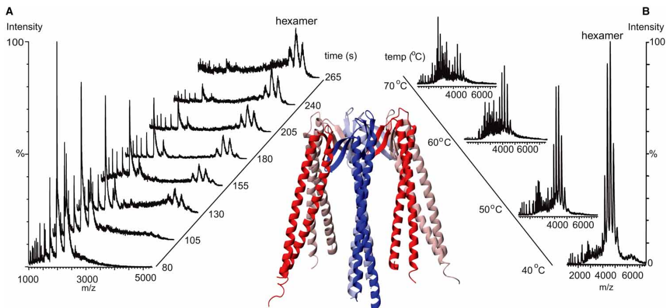
Figure 1. (A) The assembly of MtGimC from its component subunits. \alpha -Subunits (red) form a dimeric platform for assembly of the four \beta -subunits monitored in real time by MS. (B) The thermal stability of the MtGimC hexamer investigated as a function of temperature. Reproduced with permission from ref. [15]. Inset , X-ray structure of the MtGimC complex [62] from the co-ordinates 1FXK.
