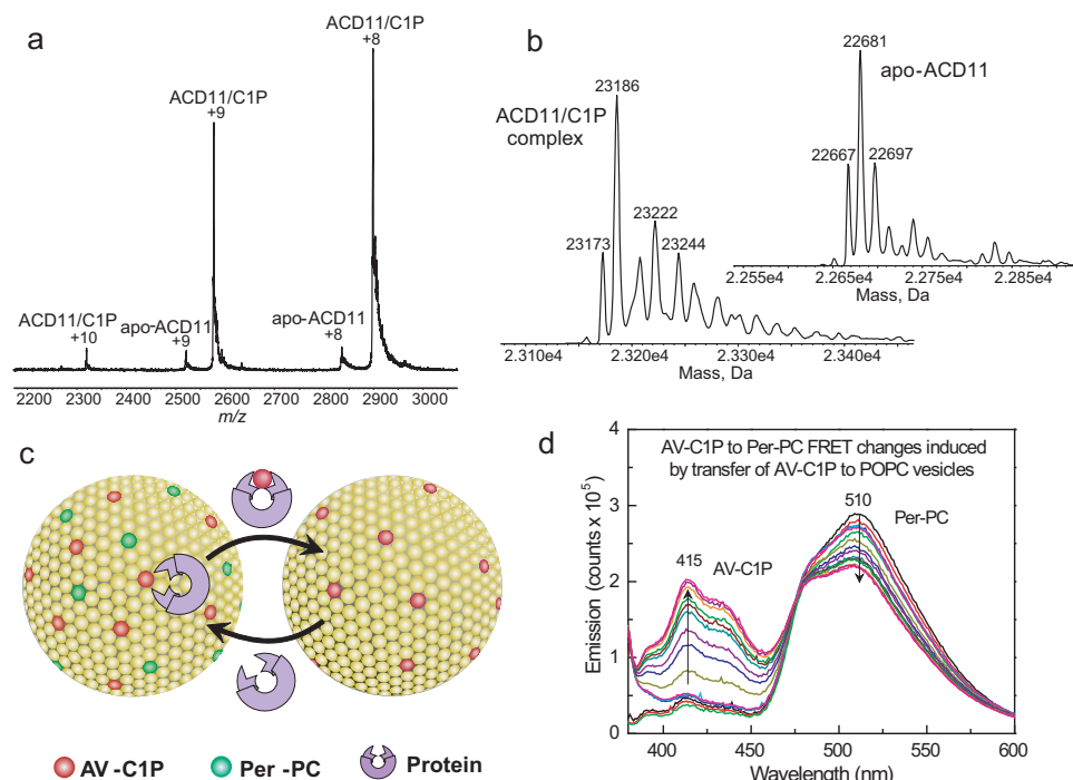
FIGURE 2. Surface electrostatics surrounding the sphingolipid liganding site in ACD11, C1P, and GLTP and sphingolipid intermembrane transfer measurement using a FRET-based assay. a , ESI-MS analysis of ACD11·C1P complex. Direct infusion under nondenaturing conditions results in two main positive charge states (+8 and +9) for the ACD11· N -octanoyl C1P complex. Traces of apo-ACD11 also are evident for the +8 and +9 charge states. The m/z label ( x axis) represents mass divided by charge number. b , the transformed spectra indicate molecular masses of 22,681 Da for apo-ACD11 and 23,186 Da for the ACD11· N -octanoyl C1P complex, confirming a single binding site for C1P. c , schematic for in vitro measurement of SL intermembrane transfer via FRET loss. In the SL source vesicle, the AV-SL fluorescence signal (energy donor; red dots) is low due to FRET involving perylenoyl-PC (energy acceptor; green dots; nontransferable lipid). Loss of FRET occurs when AV-SL is removed by protein (catalytic amount) and transferred to the excess (10-fold) POPC receiver vesicles, resulting in a time-dependent increase in AV-SL emission signal. d , spectral emission changes for AV-SL/Per-PC energy transfer pair showing FRET loss induced by transfer protein activity. AV-C1P and Per-PC are at 1 mol % in SL source vesicles. Black, red, and green traces, successive scans of SL source vesicles (2.5-min intervals) showing signal stability; blue, cyan, and magenta traces, successive scans (2.5-min intervals) after the addition of excess POPC receiver vesicles; other spectral traces show the time-dependent emission changes in AV and Per (2-min intervals) after injection of transfer protein (2 \mu g).
