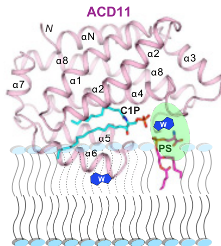
FIGURE 7. Model for putative PS-induced enhancement of ACD11. The model shows how the PS acyl chains remain embedded in the membrane while the PS headgroup ( magenta ) interacts with a putative surface site in ACD11 ( ribbon representation ) to help orient the C1P binding site to improve uptake of the C1P binding site and the membrane interaction region of ACD11.
