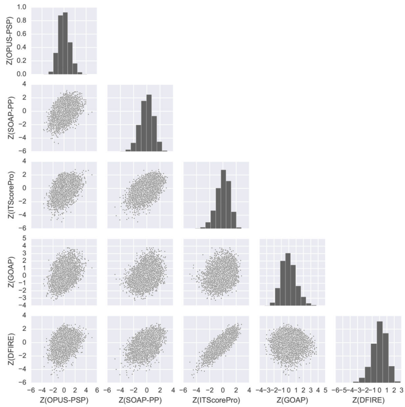
Figure 3. Single and pairwise score distributions for decoys of target T72. This is an unsuccessful decoy set example, which contains no acceptable decoys out of 9999 total.
