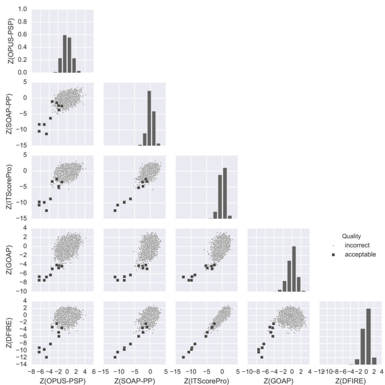
Figure 2. Single and pairwise score distributions for decoys of target T93. This decoy set is a successful example of docking, which contains ten acceptable decoys out of 9999 total. The scatter plots show pairwise score distributions. Acceptable models are shown in squares. Along the diagonal, histograms of the Z-scores of individual scores are shown.
