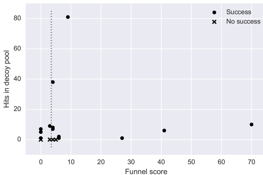
Figure 5. Prediction of decoy pool quality based on score pair distribution shape. “Funnel score” is the sum of n over all score pairs where the SCC for the n\sigma -outliers is significant ( p < 0.05 ) and greater than 0.4 (Equation 3). The dotted line indicates a minimum Funnel score of 3, which classifies 9 true positives, 4 true negatives, 2 false positives (T77 and T88), and 4 false negatives (T75, T86, T89, and T92).
