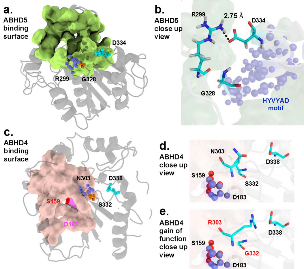
Figure 6. Shape analysis of ABHD5 and ABHD4 binding surfaces. (a) The functionally important residues D334 (cyan), R299 (slate), and G328 (orange) in spheres are spatially clustered on the predicted ABHD5 binding surface (light green). (b) A close up view shows that residues G328 and D334 are centered around R299. The model predicts the local structure of ABHD5 may be stabilized by a salt-bridge between the D334 carboxyl group (red) and the R299 guanidinium group (blue). The HYVYAD motif containing D334 is shown in blue spheres. (c) The predicted catalytic ABHD4 residues D183 (violet) and nucleophile S159 (red) form a dyad located inside the deep tunnel of the identified ABHD4 binding surface (light orange). ABHD4 N303 (slate), S332 (orange) and D338 (cyan) are spatially oriented similarly to the corresponding key residues R299, G328, and D334 in ABHD5 (a) and are situated away from the ABHD4 catalytic center S159. (d) Close up view of ABHD4 N303, S332, and D338. Note that the region occupied by N303, S332 and D338 is spatially remote from the ABHD4 catalytic residues S159 and D183 (spheres). (e) In ABHD4 N303R/S332G, R303, G332 and D338 are spatially oriented similarly to R299, G328, and D334 in ABHD5 (b), conferring on ABHD4 N303R/S332G the ability to activate ATGL.
