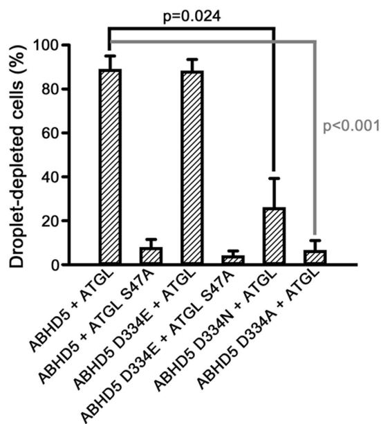
Figure 7. ABHD5 lipolysis activation requires a negatively charged amino acid at position 334. Cos7 cells were transfected with wild-type ABHD5 or the indicated ABHD5 D334 mutant constructs then lipid loaded and scored for lipid droplet content by blinded analysis. Results are mean \pm SEM from three independent experiments.
