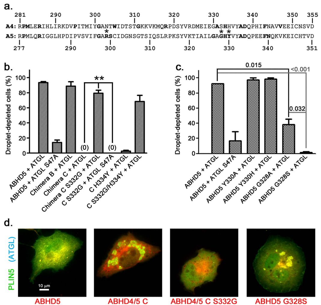
Figure 2. ABHD5 G328 is essential for ATGL activation. (a) Homology analysis of vertebrate ABHD4 and ABHD5 paralogs. Identical residues in all vertebrate homologs of each protein are indicated in bold, based on analysis of proteins in the NCBI database as of May 2016. Asterisks indicate ABHD5 identical residues not conserved between ABHD4 and ABHD5. (b) Chimera C S332G activates lipolysis in Cos7 cells. ** p < 0.01 . (c) ABHD5 G328S does not activate lipolysis. Values are means \pm SEM from three independent experiments. (d) Representative images of ABHD mutant transfected Cos7 cells. Scale bar = 10 \mu m.
