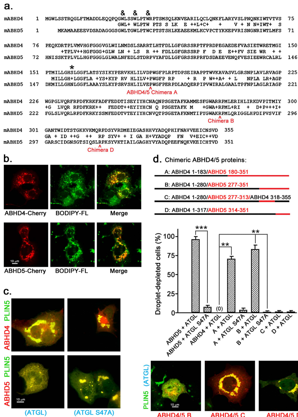
Figure 1. Chimeric ABHD4 1–280/ABHD5 277–351 activates ATGL-dependent lipolysis.
