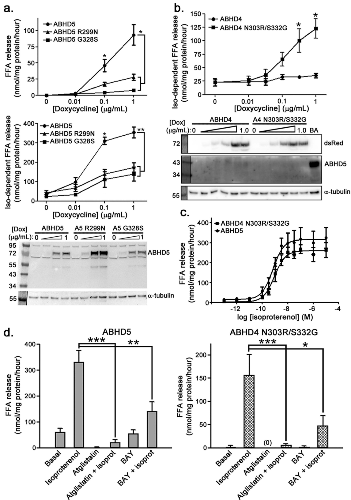
Figure 4. Characterization of loss-of-function and gain-of-function ABHD proteins in ABHD5-null BAs. Doxycycline-inducible ABHD-mCherry proteins were expressed in a BA cell line in which endogenous ABHD5 was silenced by shRNA. In the immunoblots shown in 4a and 4b, it should be noted that the mCherry tag shifts the ABHD protein molecular weight from \sim 43 kDa for endogenous ABHD5 to \sim 72 kDa for the mCherry-tagged protein. (a) ABHD5 R299N and G328S mutations inhibit basal (top panel) and isoproterenol-stimulated lipolysis (middle panel). Values are mean \pm SEM from three or more independent experiments. Representative
