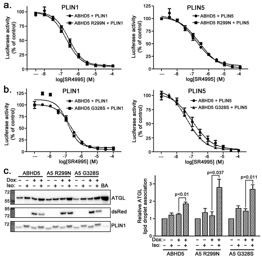
Figure 5. Effect of ABHD5 loss-of-function mutations on ligand binding, association with PLIN proteins, and ATGL translocation. (a,b) ABHD5 loss-of-function mutations do not affect ligand binding or association with PLIN proteins. Mean \pm SD from one of at least two independent experiments with similar results is shown. (c) ABHD5 loss-of-function mutations do not affect ATGL translocation to LDs in BA cells. LDs were isolated from the indicated differentiated BA cell lines that were treated with 100 nM isoproterenol (or untreated control cells) for 30 mins. Densitometric analysis (mean \pm SEM) in right panel is based on three independent experiments.
