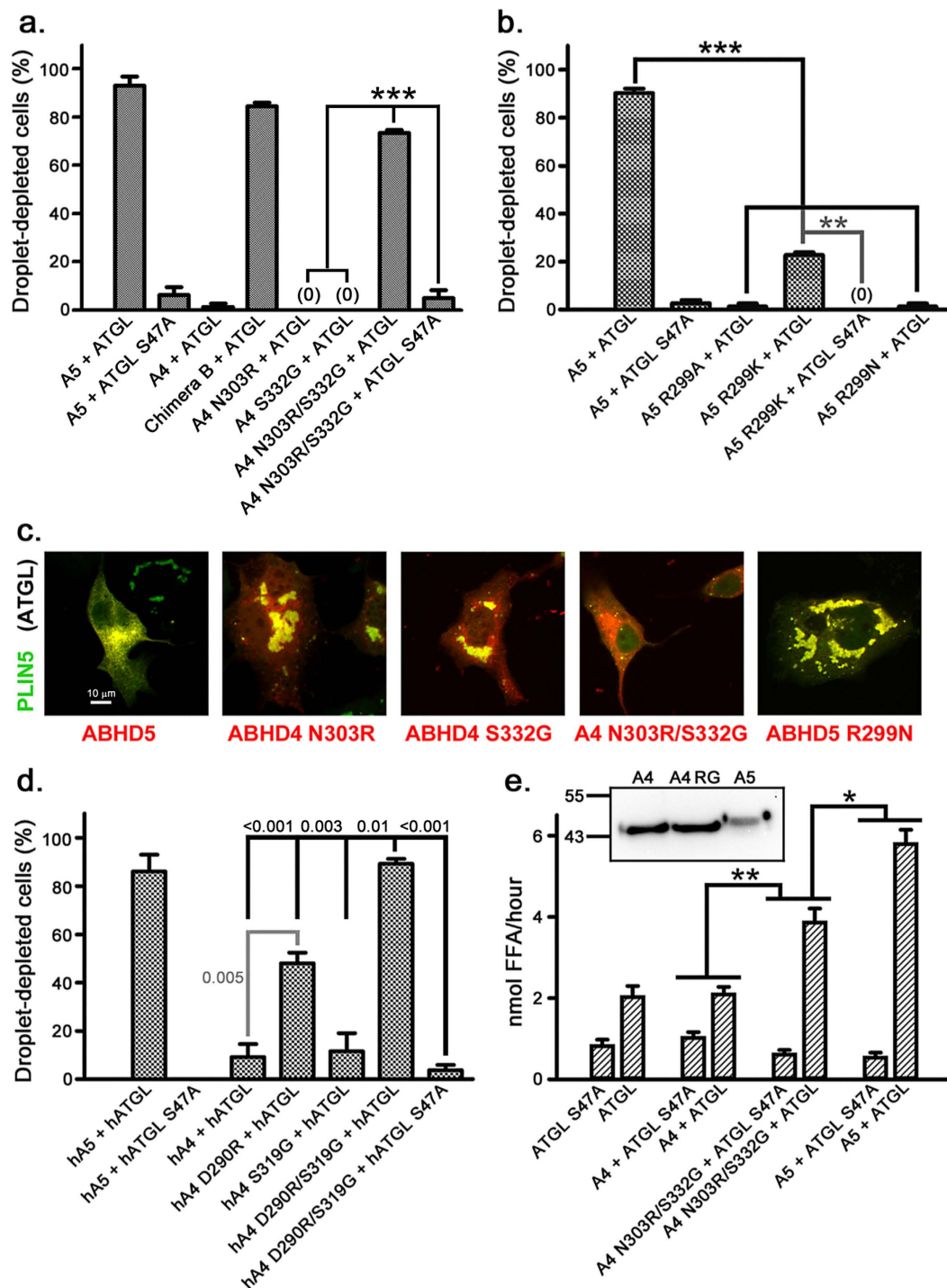
Figure 3. ABHD5 R299 is essential for ATGL activation. (a) ABHD4 N303R/S332G activates ATGL-dependent lipolysis in transfected Cos7 cells. (b) ABHD5 R299N does not activate lipolysis. (c) Representative images of ABHD mutant transfected Cos7 cells. Scale bar = 10 \mu m. (d) Human ABHD4 D290R/S319G activates lipolysis. (e) Partially purified ABHD4 N303R/S332G activates lipolysis in artificial LDs. Inset shows strep tag immunoblot of relative ABHD protein levels in assay. For (a,b,d,e), values are means \pm SEM from three independent experiments. * p < 0.05; ** p < 0.01; *** p < 0.001.
